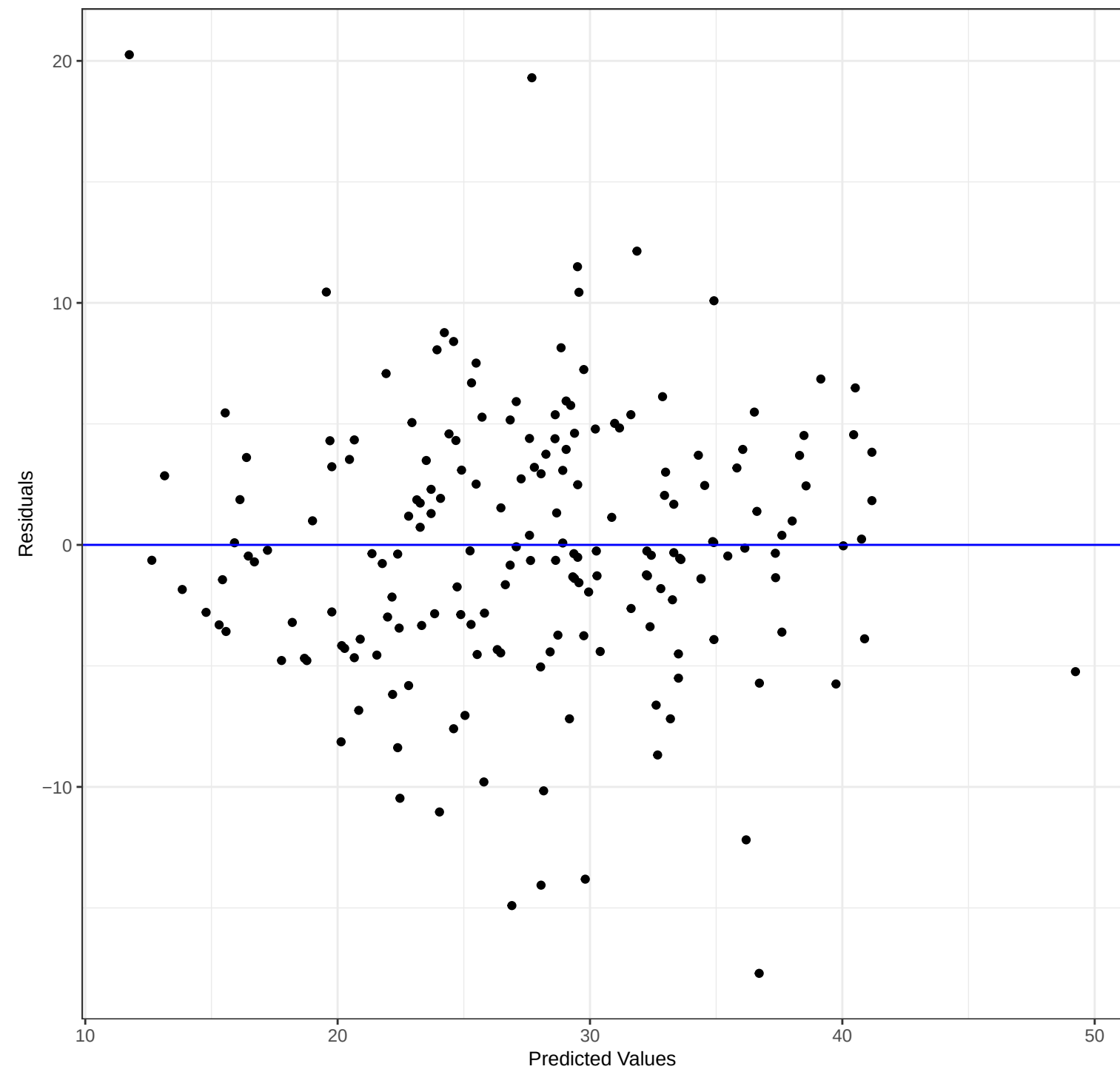
Residual Plot
