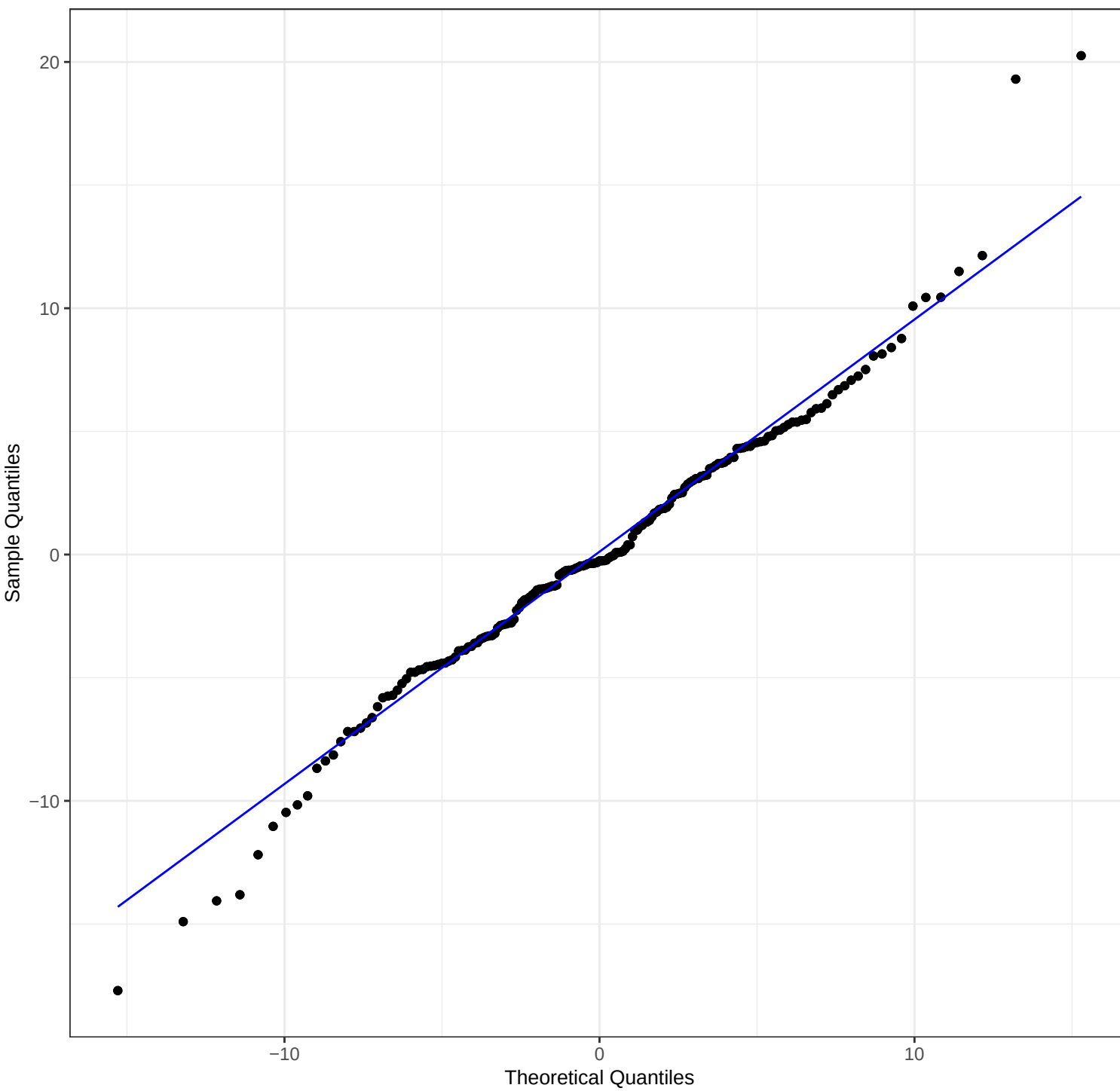
Q-Q Plot
