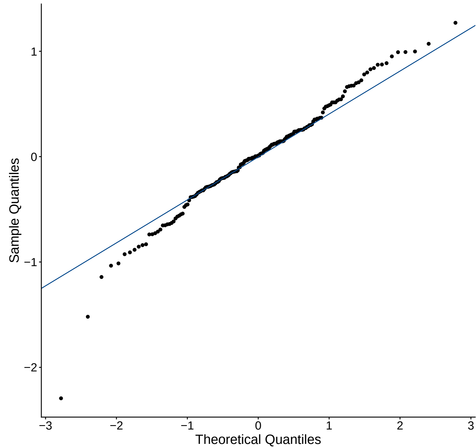
Q-Q Plot
