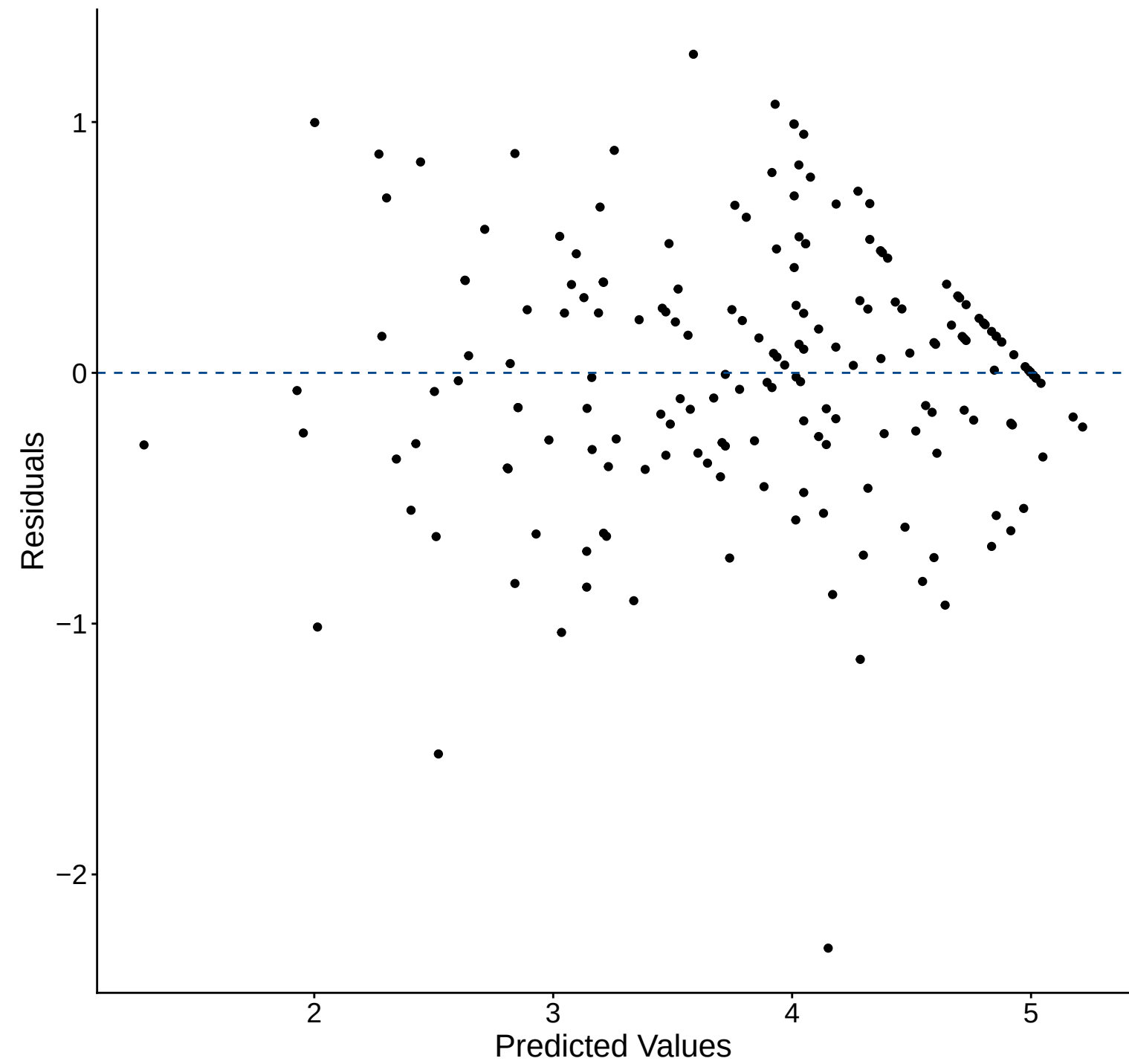
Residual Plot
