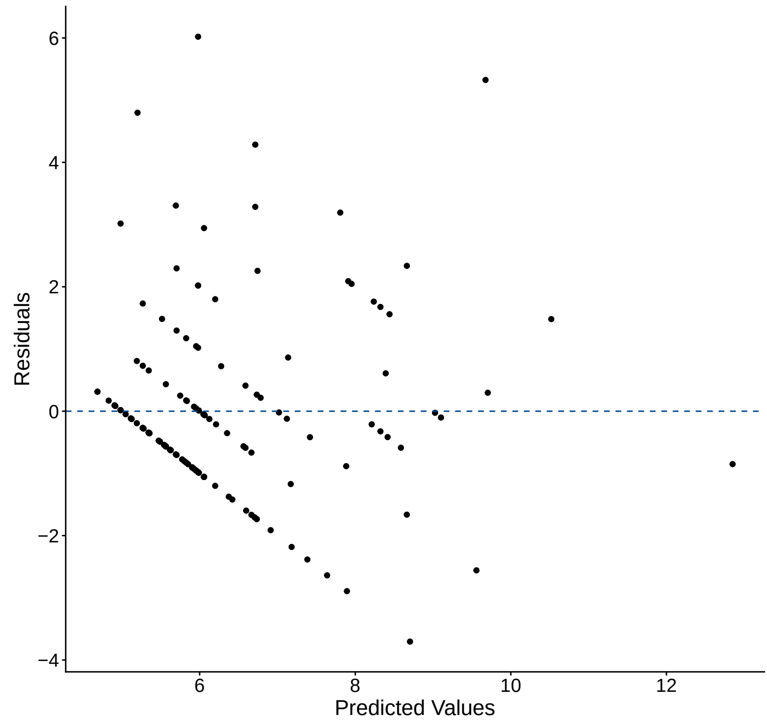
Residual Plot
