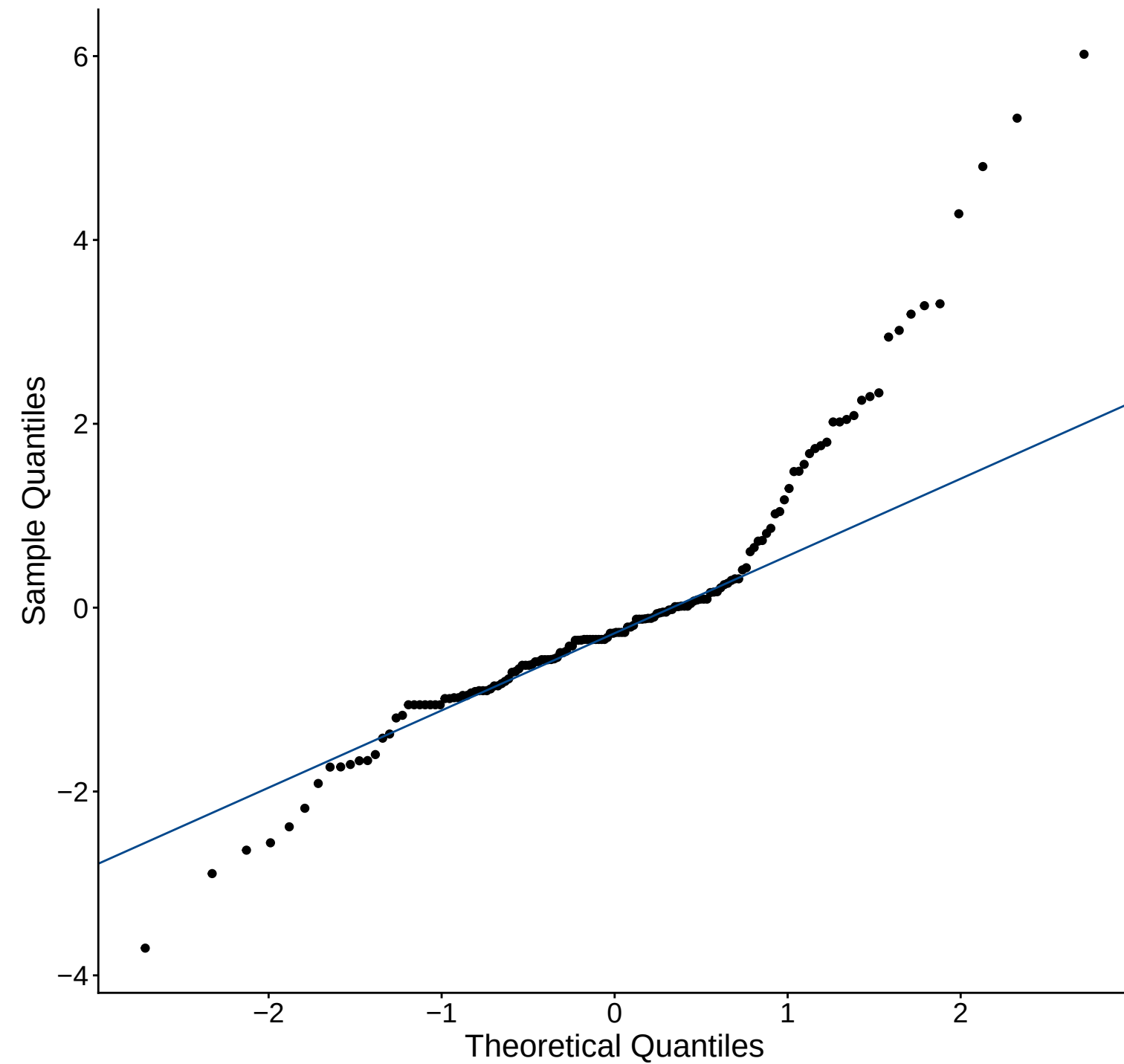
Q-Q Plot
