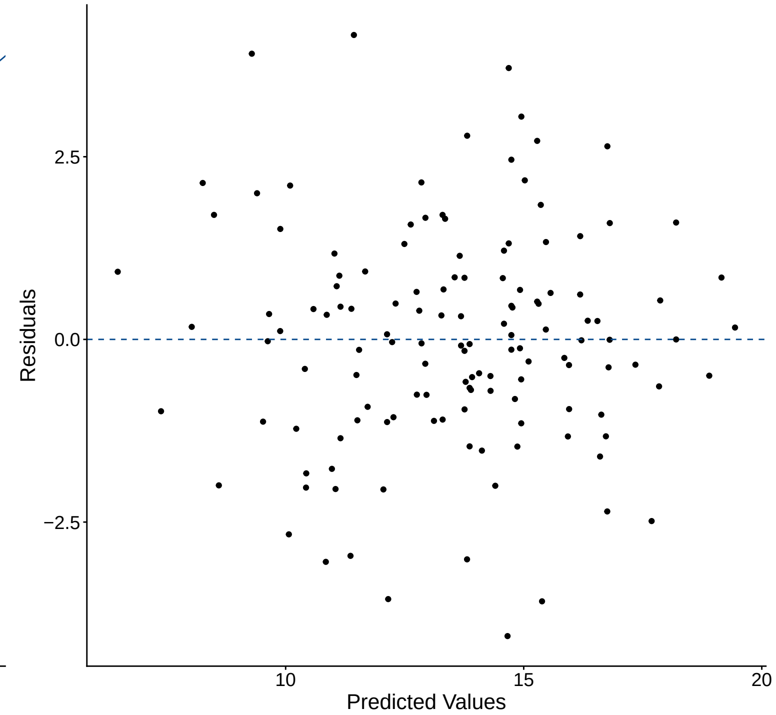
Residual Plot
