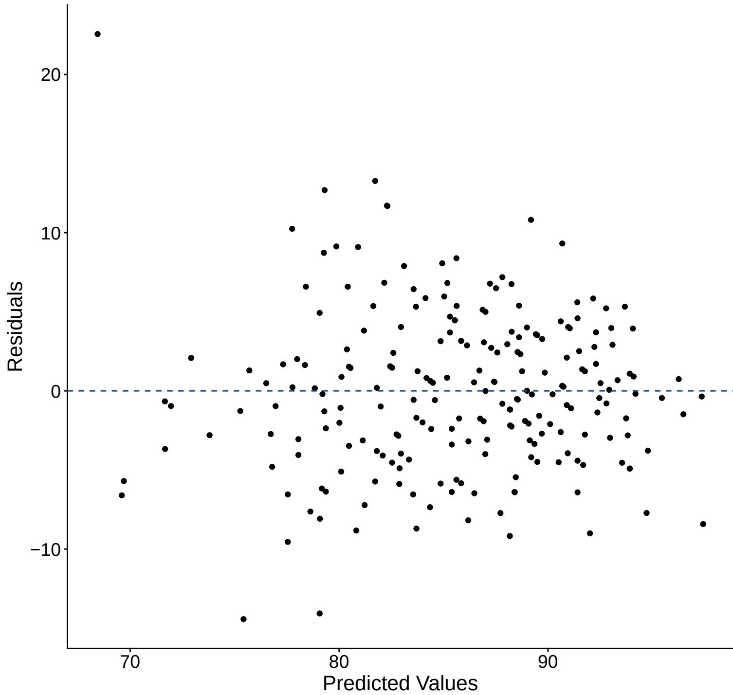
Residual Plot
