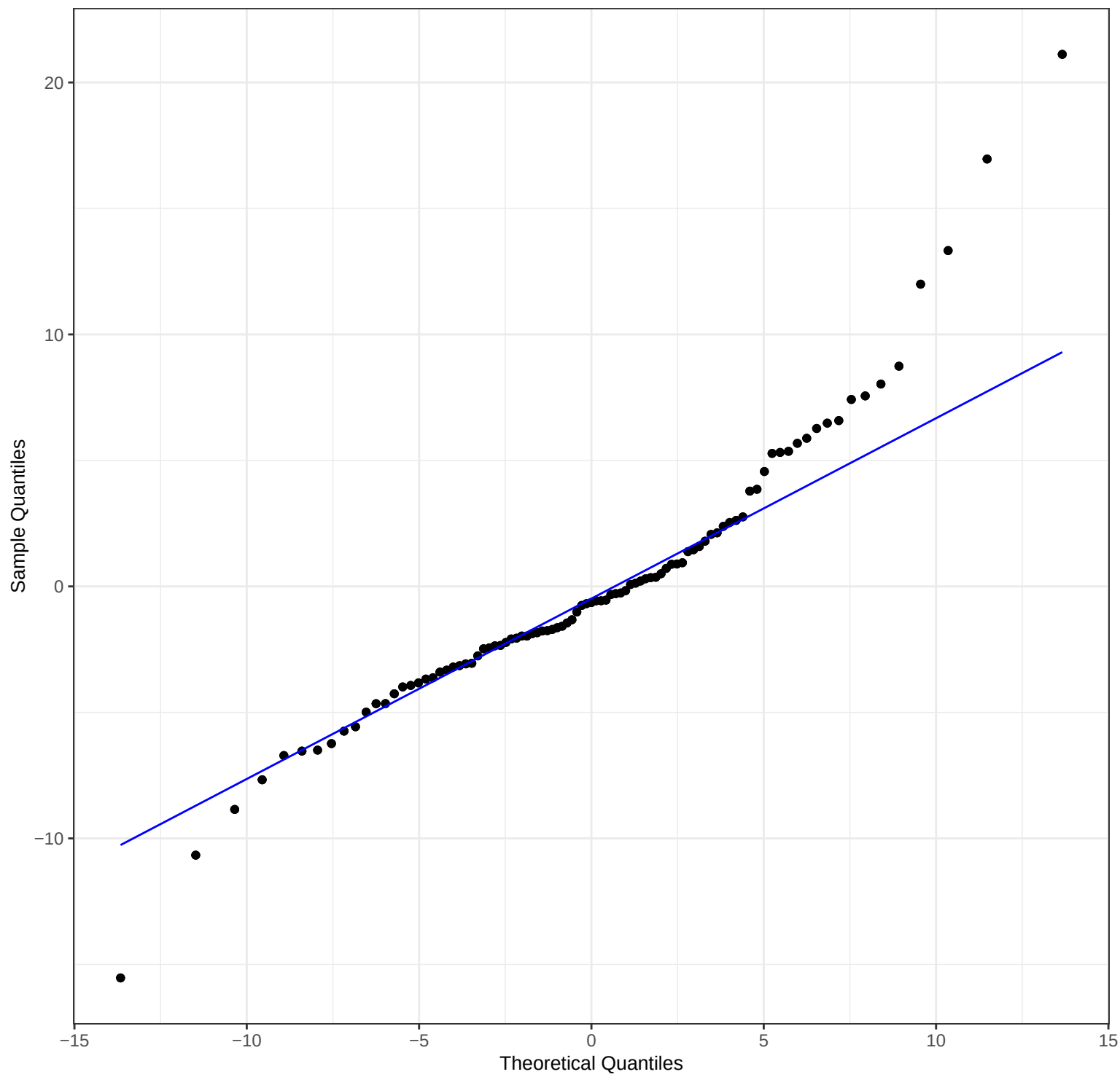
Q-Q Plot
