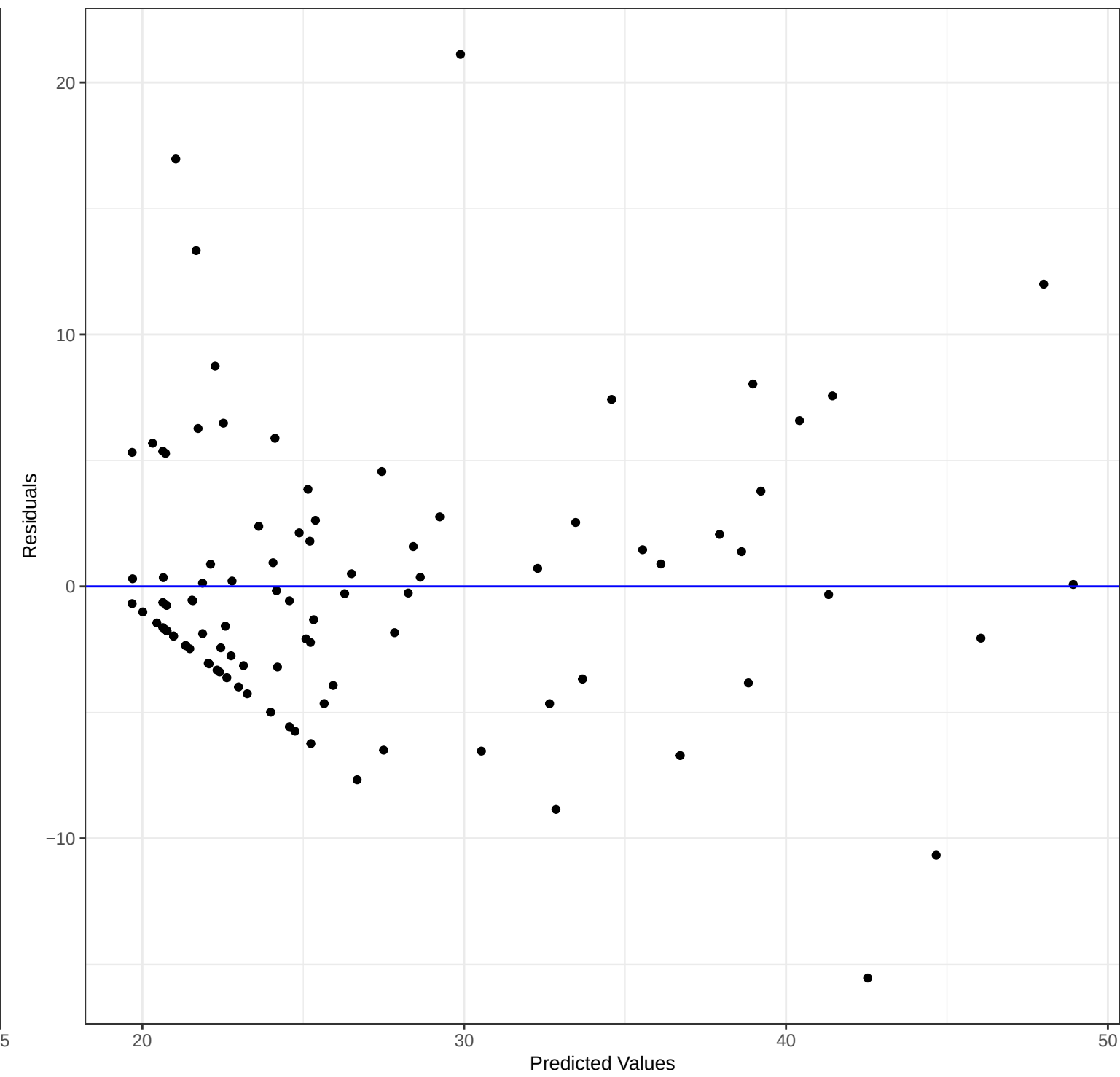
Residual Plot
