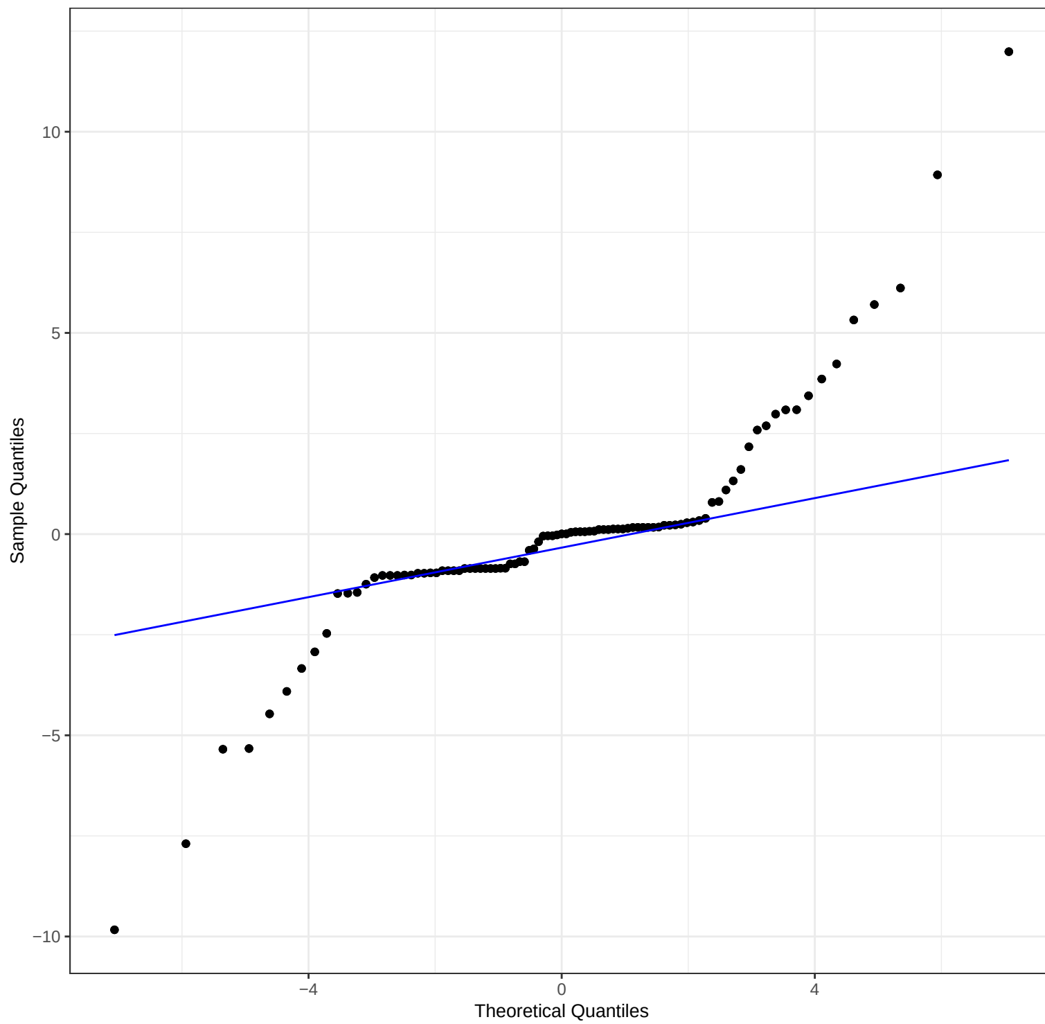
Q-Q Plot
