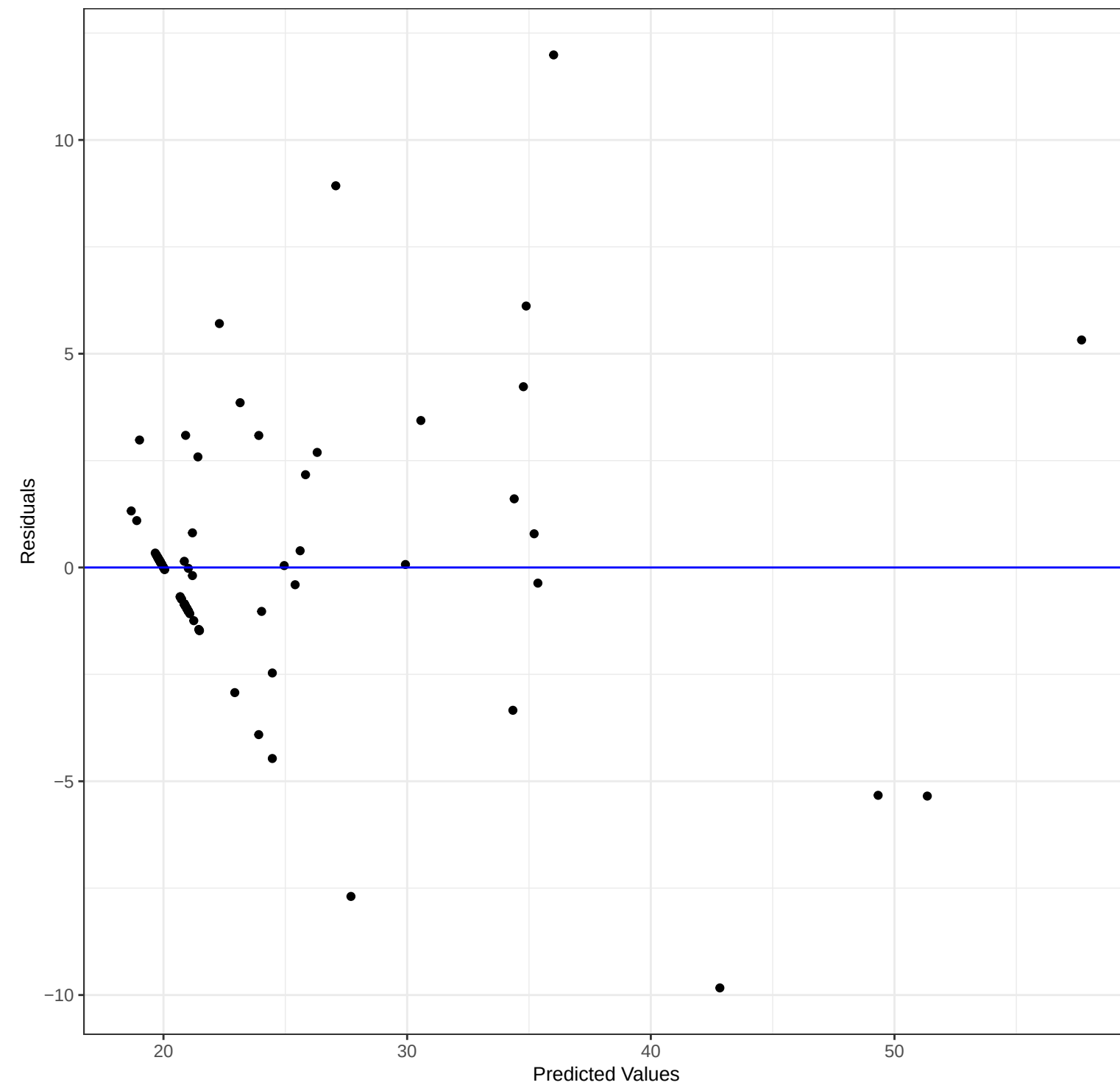
Residual Plot
