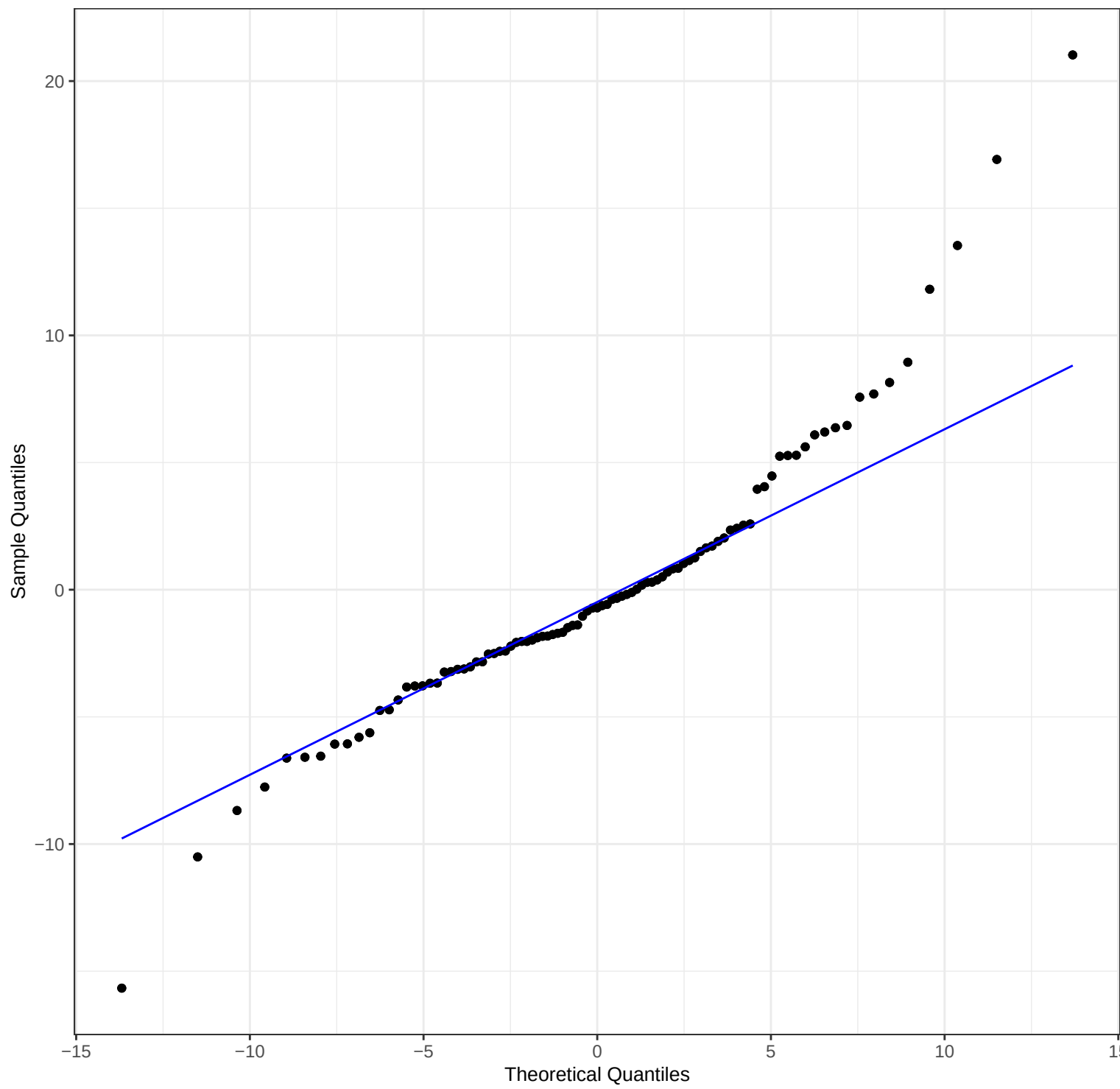
Q-Q Plot
