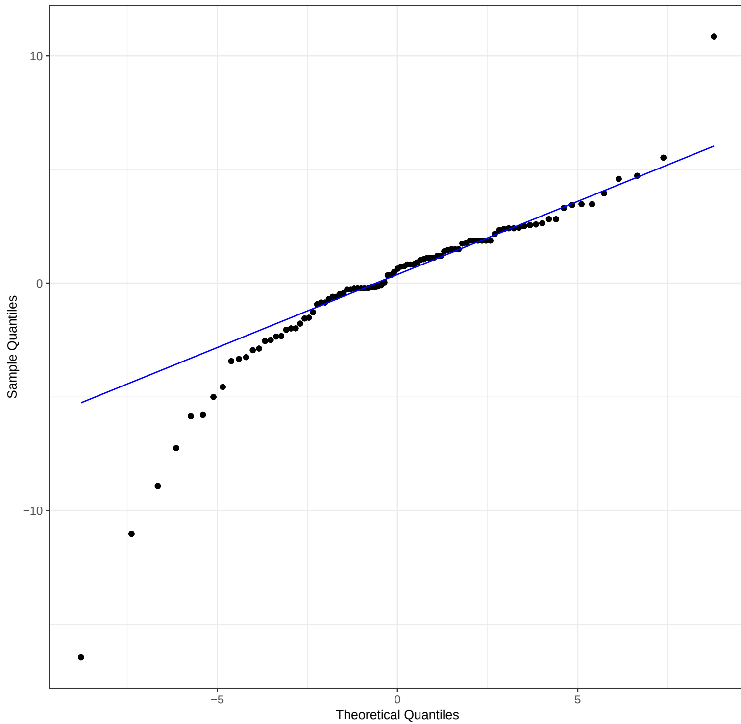
Q-Q Plot
