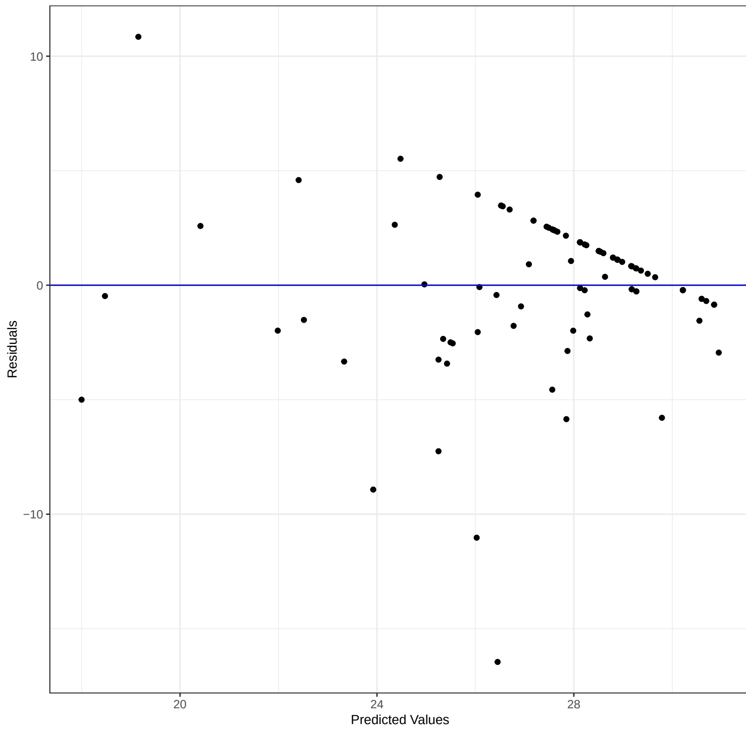
Residual Plot
