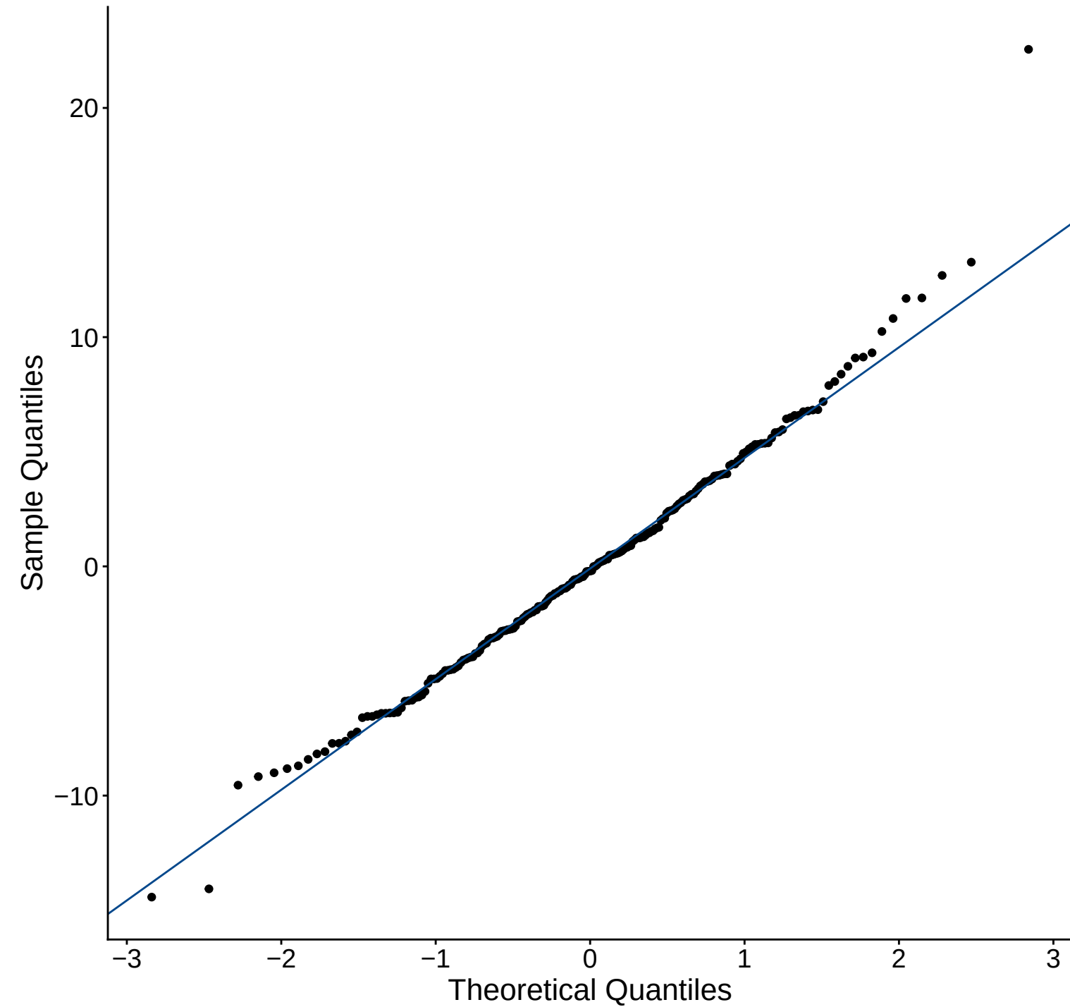
Q-Q Plot
