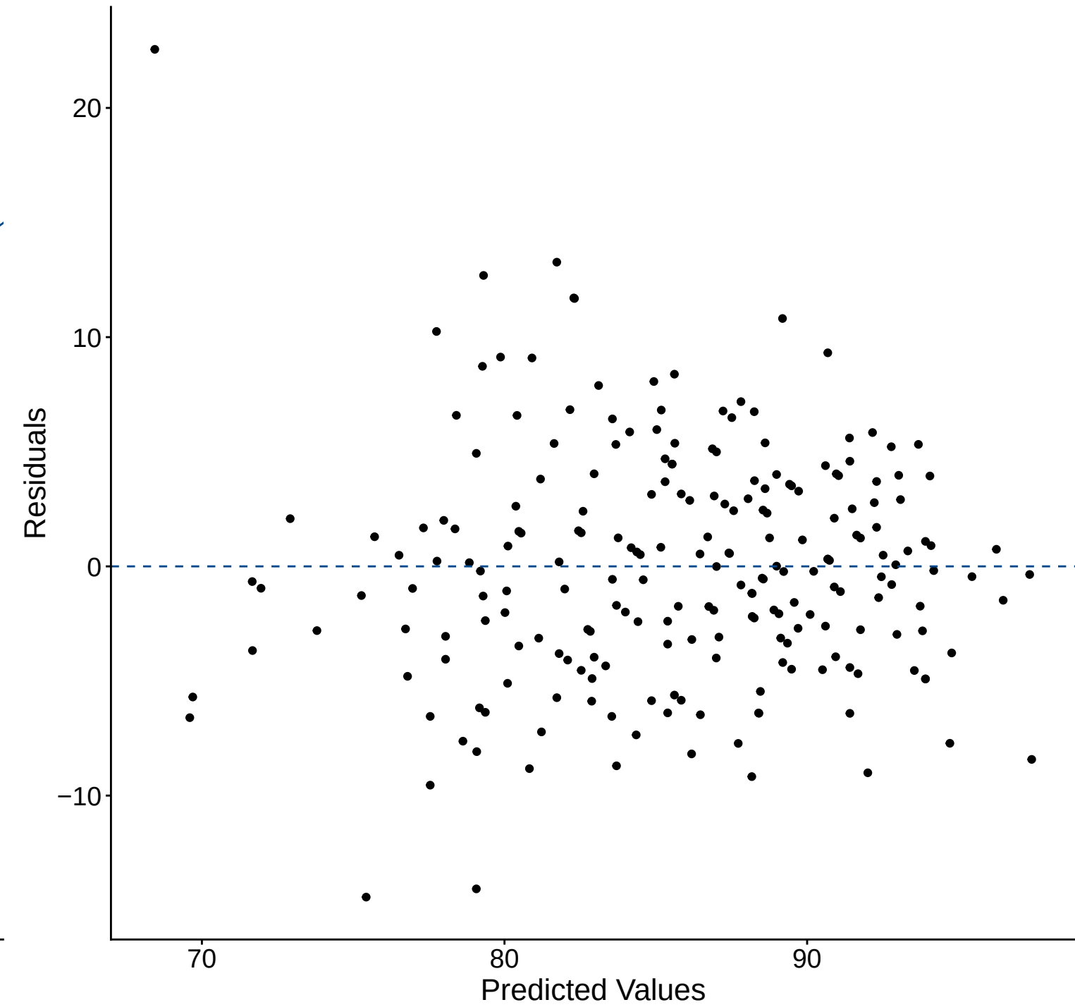
Residual Plot
