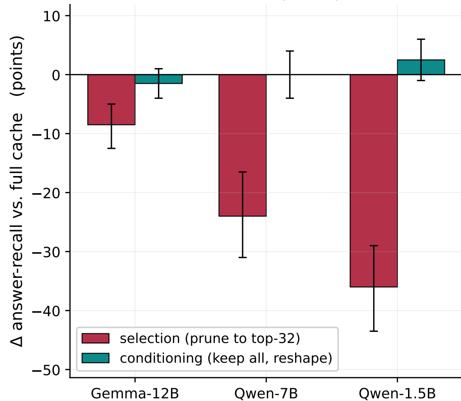
SQuAD (single-hop)
