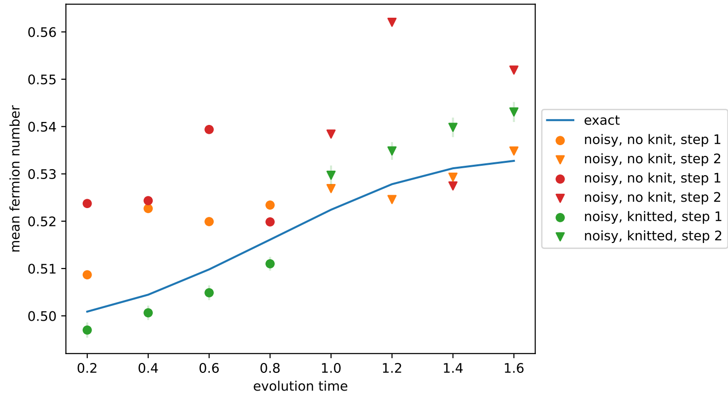
Time Evolution of Mean Fermion Number
