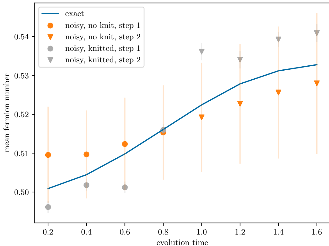
Time Evolution of Mean Fermion Number
