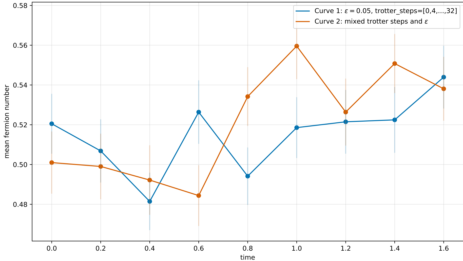
Trotter Comparison
