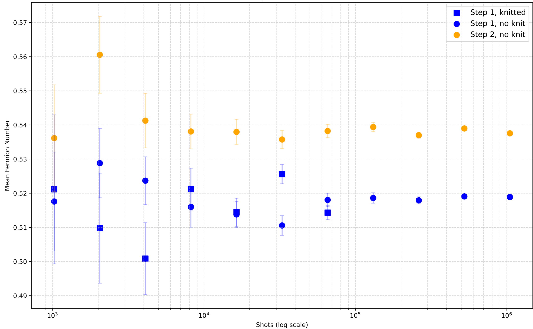
Noiseless Trotter Steps: Fermion Number vs Shots with Error Bars (Epsilon = 0.8)
