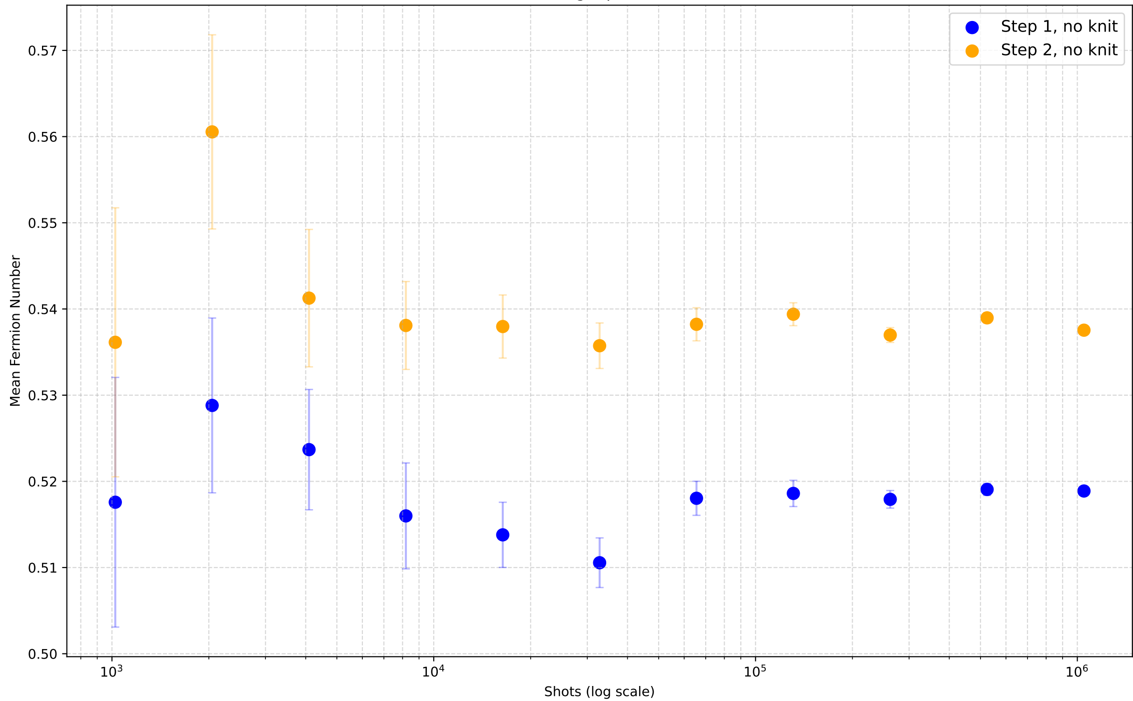
Noiseless Trotter Steps: Fermion Number vs Shots (No Knitting, Epsilon = 0.8)
