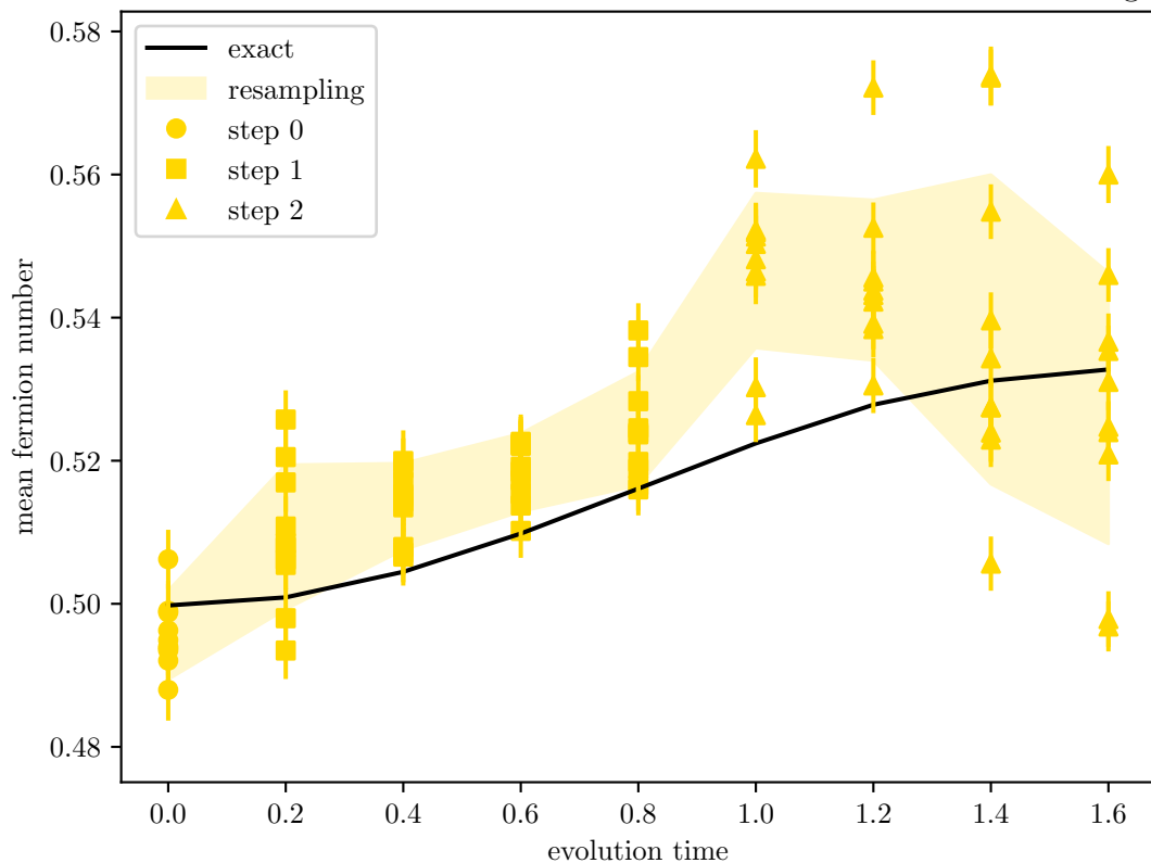
Time Evolution of Mean Fermion Number without Circuit Knitting
