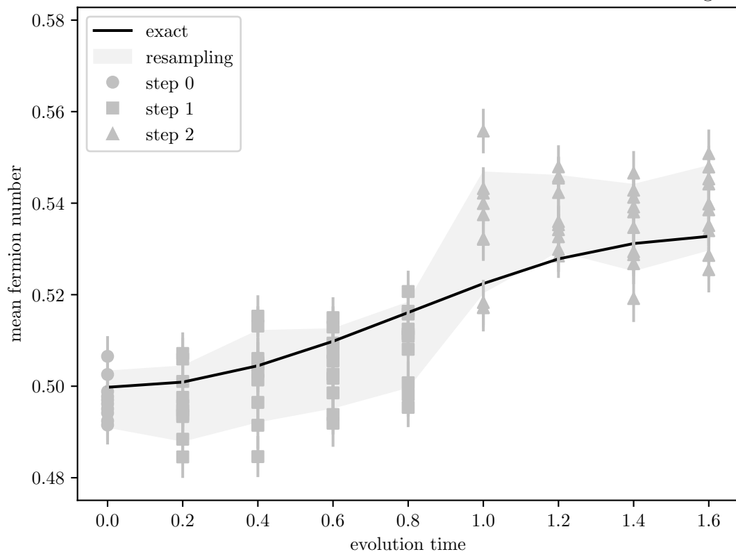
Time Evolution of Mean Fermion Number with Circuit Knitting
