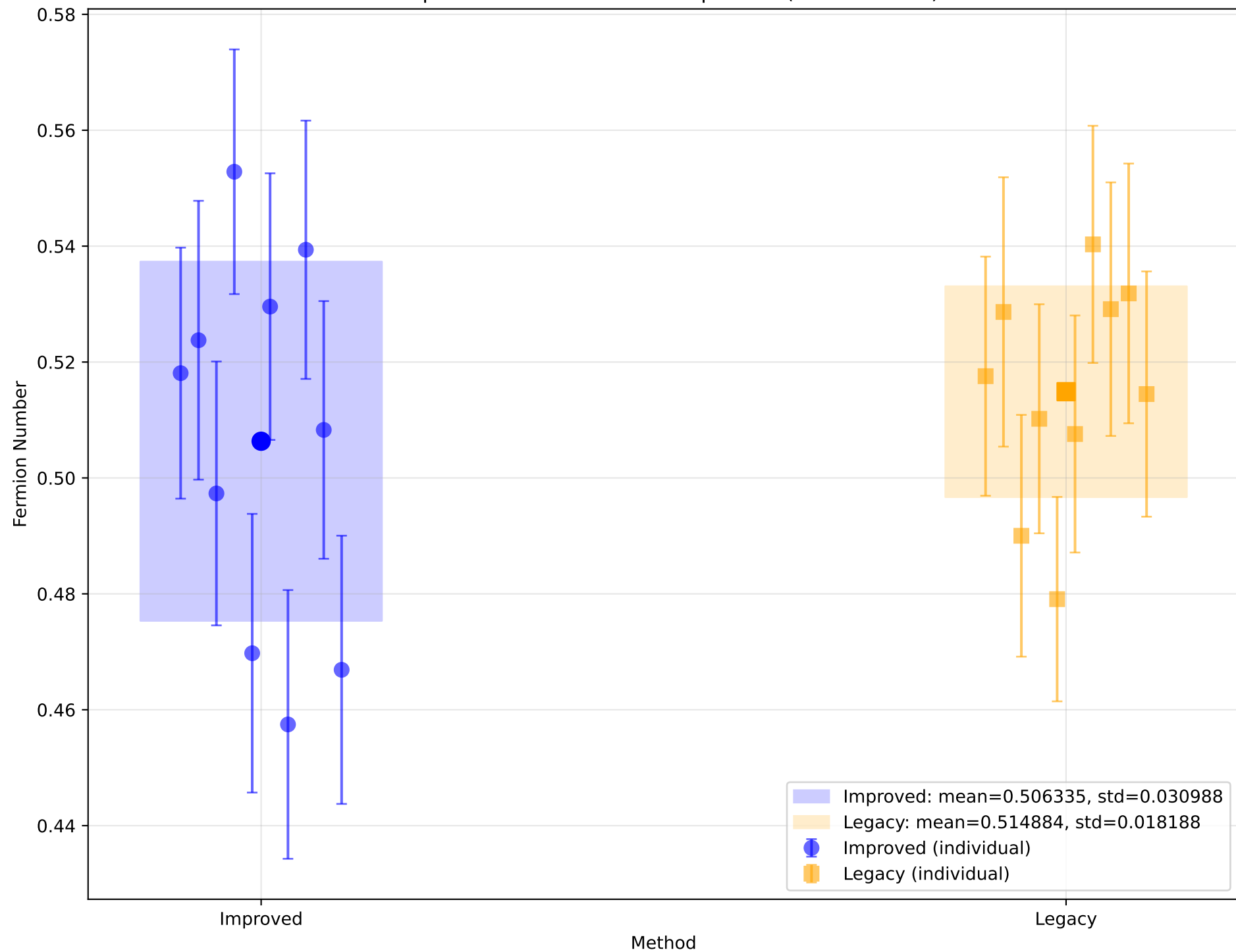
Step 1: Fermion Number Comparison (10 runs each)
