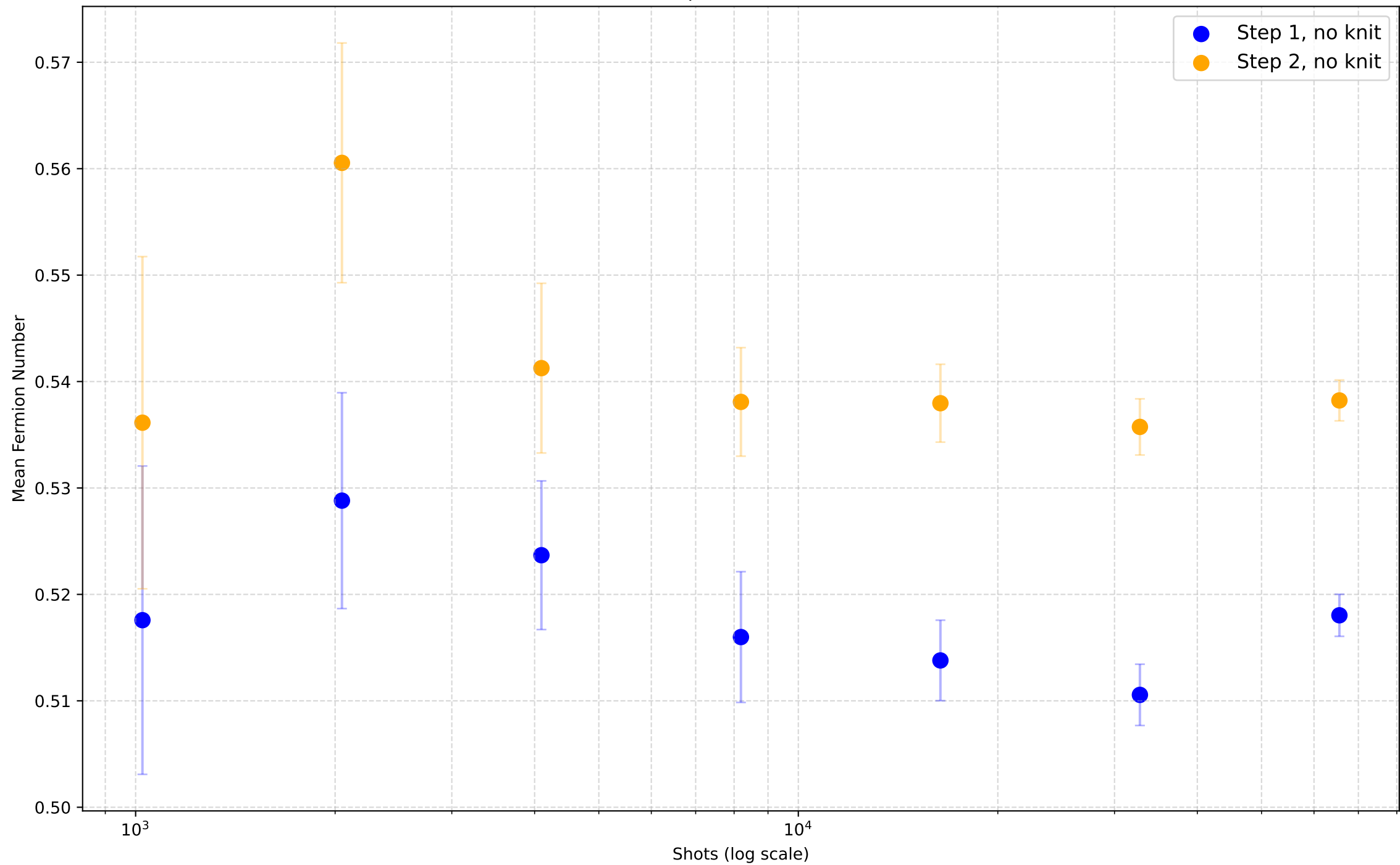
Noiseless Trotter Steps: Fermion Number vs Shots (Epsilon = 0.8)
