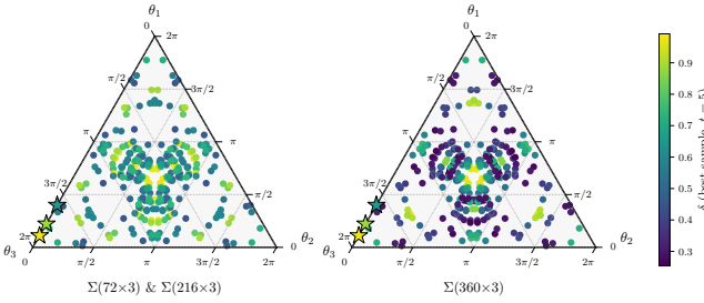
FIG. 4. \delta on the SU(3) maximal torus at t = 5 . Each panel shows the 50 random-diagonal extensions of Section V.4, S_3 -symmetrized to six copies each (300 points per panel). The left panel, labeled \Sigma(72 \times 3) & \Sigma(216 \times 3) , reports the \delta values that are bit-for-bit identical on the two smaller \Sigma -series groups; the right panel reports \Sigma(360 \times 3) . Red stars mark the three structured rational-angle extensions P(2\pi/9) , P(\pi/9) , P(2\pi/5) from Table III, colored by their own \delta on each group; they sit on the \theta_1 = 0 edge because each has the form \text{diag}(1, e^{i\theta}, e^{-i\theta}) .
