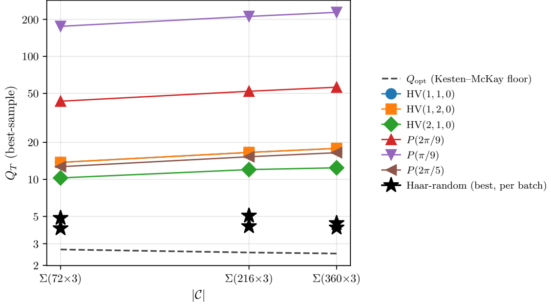
FIG. 2. Q_T across the three \Sigma -series base groups at d = 3 , t = 10 , for every extension in the panel of Table III. The dashed line is the Kesten–McKay floor Q_{\text{opt}} of Eq. (5); rational-angle diagonal and Howard–Vala extensions run nearly parallel to it at a factor \sim 3 –70 offset (Finding 2), while arbitrary-SU(3) extensions (stars) approach Q_{\text{opt}} as |\mathcal{C}| grows (Finding 3). The HV(1, 1, 0) and HV(1, 2, 0) markers coincide at every |\mathcal{C}| because the two gates are Clifford-equivalent at d = 3 (Eq. (7)).
