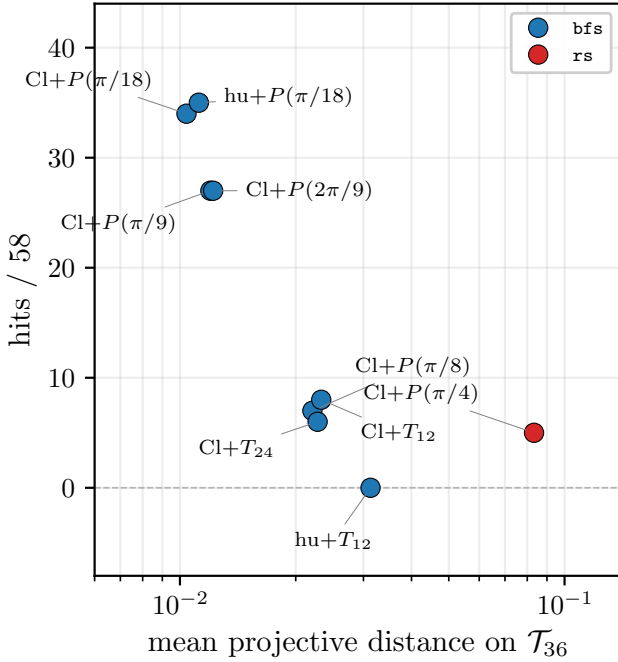
FIG. 5. DSA \Sigma(36 \times 3) target-family coverage from Table V: hits/58 versus mean projective distance on \mathcal{T}_{36} at BFS depth 15, \varepsilon = 10^{-2} . Canonical Clifford+ T (red, rs_exact certified) sits bottom-right with the largest mean distance and only 5 hits. Rational-angle P(k\pi/18) extensions (blue, bfs_estimate ) cluster top-left with many hits at an order of magnitude smaller distance; super-golden T_{12}/T_{24} rows fall in between despite saturating Q_{\text{opt}} (Section IV). The visual separation matches the 6.8\times headline.
