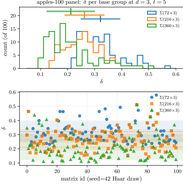
FIG. 3. Apples-to-apples Haar panel at N = 100 matrices on the three d = 3 \Sigma -series base groups. Matrix id k \in \{0, \dots, 99\} labels apple k , the k -th Haar-SU(3) draw from seed = 42; ids 0–9 coincide with the ten-matrix subset of Table IV. Top: overlaid \delta histograms. Bottom: per-matrix \delta for each group. The monotone reduction \mu_{216} > \mu_{648} > \mu_{1080} predicted by Finding 3 is resolved at \sim 5.7\sigma/\sqrt{N} ; the single apple05 outlier visible as the \Sigma(360 \times 3) peak near \delta \simeq 0.44 is the one that inverted the ten-matrix ordering in Table IV.
