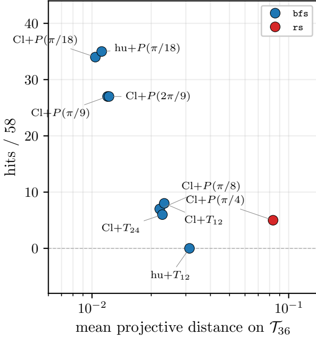
FIG. 4. DSA \Sigma(36 \times 3) target-family coverage from Table IV: hits/58 versus mean projective distance on \mathcal{T}_{36} at BFS depth 15, \varepsilon = 10^{-2} . Canonical Clifford+ T (red, rs_exact certified) sits bottom-right with the largest mean distance and only 5 hits. Rational-angle P(k\pi/18) extensions (blue, bfs_estimate ) cluster top-left with many hits at an order of magnitude smaller distance; super-golden T_{12}/T_{24} rows fall in between despite saturating Q_{\text{opt}} (Section IV). The visual separation matches the 6.8\times headline.
