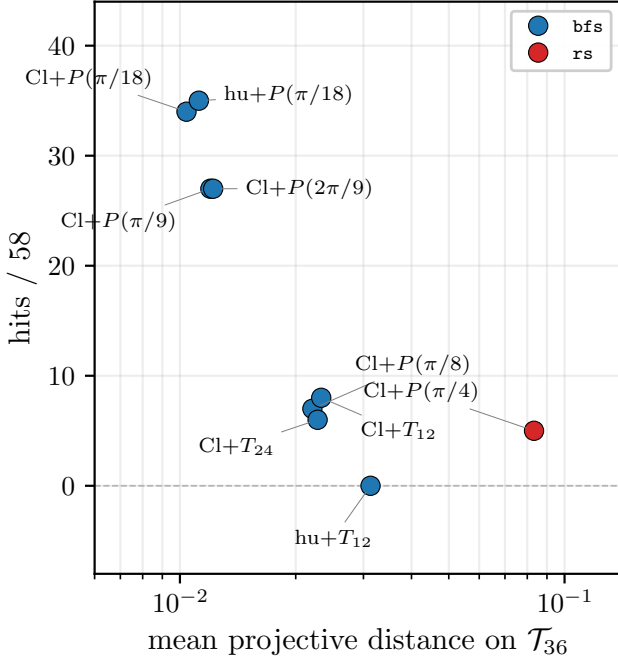
FIG. 4. DSA \Sigma(36 \times 3) target-family coverage from Table IV: hits/58 versus mean projective distance on T_{36} at BFS depth 15, \varepsilon = 10^{-2} . Canonical Clifford+ T (red, rs_exact certified) sits bottom-right with the largest mean distance and only 5 hits. Rational-angle P(k\pi/18) extensions (blue, bfs_estimate ) cluster top-left with many hits at an order of magnitude smaller distance; super-golden T_{12}/T_{24} rows fall in between despite saturating Q_{opt} (Section IV). The visual separation matches the 6.8\times headline.
