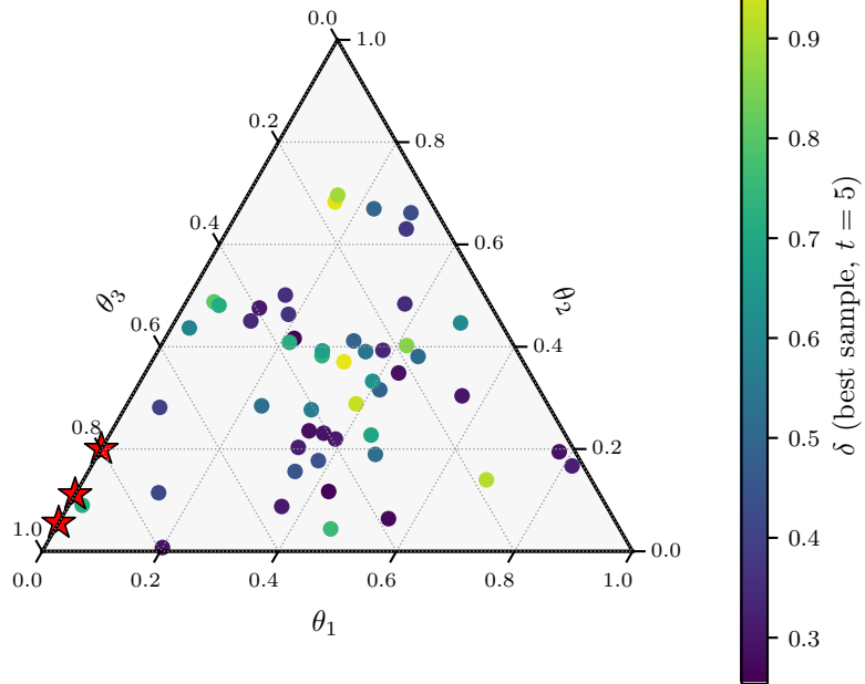
\Sigma(360 \times 3)
