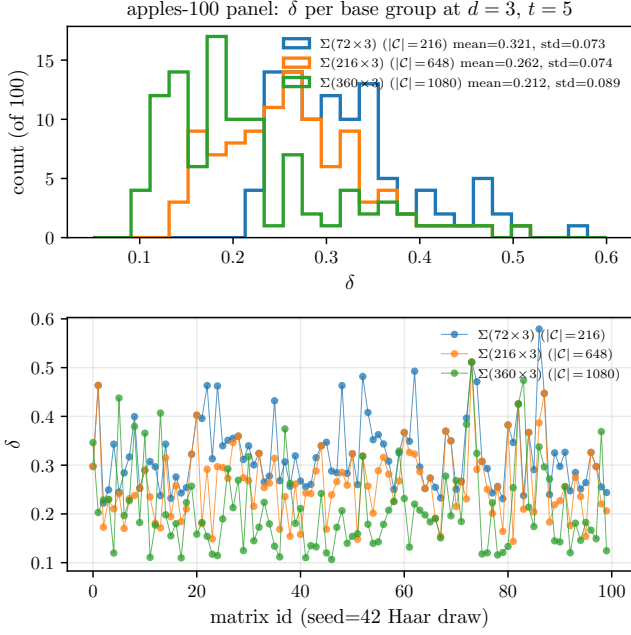
FIG. 2. Apples-to-apples Haar panel at N = 100 matrices (seed = 42) on the three d = 3 \Sigma -series base groups. Top: overlaid \delta histograms. Bottom: per-matrix \delta for each group; matrix id 0–9 coincides with the ten-matrix subset of Table III. The monotone reduction \mu_{216} > \mu_{648} > \mu_{1080} predicted by Finding 3 is now resolved at \sim 5.7\sigma/\sqrt{N} ; the single apple05 outlier visible as the \Sigma(360 \times 3) peak near \delta \simeq 0.44 is the one that inverted the ten-matrix ordering in Table III.
