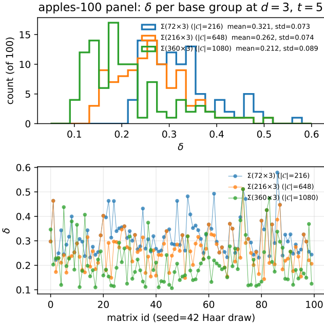
FIG. 2. Apples-to-apples Haar panel at N = 100 matrices ( seed = 42 ) on the three d = 3 \Sigma -series base groups. Top: overlaid \delta histograms. Bottom: per-matrix \delta for each group; matrix id 0–9 coincides with the ten-matrix subset of Table III. The monotone reduction \mu_{216} > \mu_{648} > \mu_{1080} predicted by Finding 3 is now resolved at \sim 5.7\sigma/\sqrt{N} ; the single apple05 outlier visible as the \Sigma(360 \times 3) peak near \delta \simeq 0.44 is the one that inverted the ten-matrix ordering in Table III.
