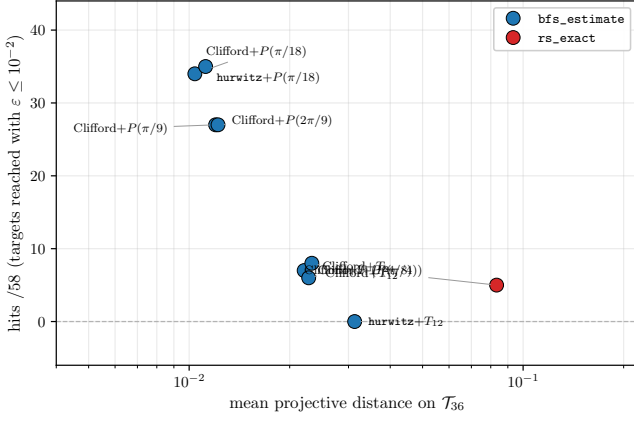
FIG. 4. DSA \Sigma(36 \times 3) target-family coverage from Table IV: hits/58 versus mean projective distance on \mathcal{T}_{36} at BFS depth 15, \varepsilon = 10^{-2} . Canonical Clifford+ T (red, rs_exact certified) sits bottom-right with the largest mean distance and only 5 hits. Rational-angle P(k\pi/18) extensions (blue, bfs_estimate ) cluster top-left with many hits at an order of magnitude smaller distance; super-golden T_{12}/T_{24} rows fall in between despite saturating Q_{\text{opt}} (Section IV). The visual separation matches the 6.8 \times headline.
