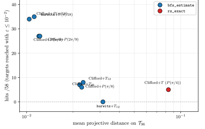
FIG. 4. DSA \Sigma(36 \times 3) target-family coverage from Table IV: hits/58 versus mean projective distance on \mathcal{T}_{36} at BFS depth 15, \varepsilon = 10^{-2} . Canonical Clifford+ T (red, rs_exact certified) sits bottom-right with the largest mean distance and only 5 hits. Rational-angle P(k\pi/18) extensions (blue, bfs_estimate ) cluster top-left with many hits at an order of magnitude smaller distance; super-golden T_{12}/T_{24} rows fall in between despite saturating Q_{\text{opt}} (Section IV). The visual separation matches the 6.8\times headline.
