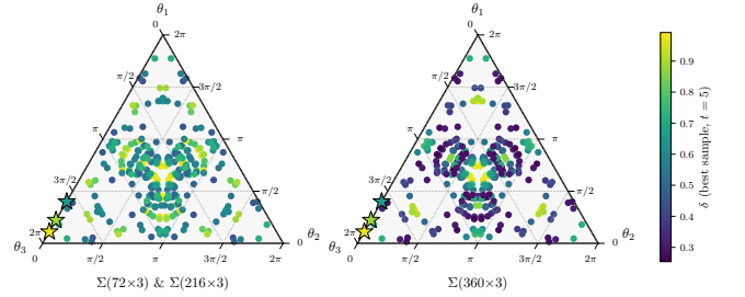
FIG. 4. \delta on the SU(3) maximal torus at t = 5 . Each panel shows the 50 random-diagonal extensions of Section V.4, S_3 -symmetrized to six copies each (300 points per panel). The left panel, labeled \Sigma(72 \times 3) & \Sigma(216 \times 3) , reports the \delta values that are bit-for-bit identical on the two smaller \Sigma -series groups; the right panel reports \Sigma(360 \times 3) . Red stars mark the three structured rational-angle extensions P(2\pi/9) , P(\pi/9) , P(2\pi/5) from Table III, colored by their own \delta on each group; they sit on the \theta_1 = 0 edge because each has the form \text{diag}(1, e^{i\theta}, e^{-i\theta}) .
