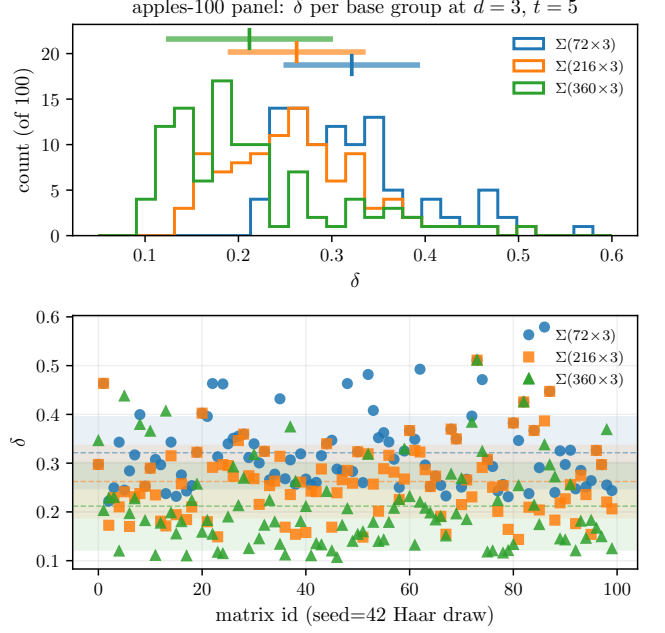
FIG. 3. Apples-to-apples Haar panel at N = 100 matrices on the three d = 3 \Sigma -series base groups. Matrix id k \in \{0, \dots, 99\} labels apple k , the k -th Haar- SU(3) draw from seed = 42; ids 0–9 coincide with the ten-matrix subset of Table IV. Top: overlaid \delta histograms. Bottom: per-matrix \delta for each group. The monotone reduction \mu_{216} > \mu_{648} > \mu_{1080} predicted by Finding 3 is resolved at \sim 5.7\sigma/\sqrt{N} ; the single apple05 outlier visible as the \Sigma(360 \times 3) peak near \delta \simeq 0.44 is the one that inverted the ten-matrix ordering in Table IV.
