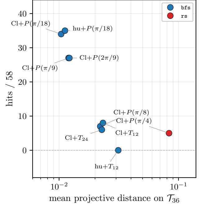
FIG. 5. DSA \Sigma(36 \times 3) target-family coverage from Table V: hits/58 versus mean projective distance on \mathcal{T}_{36} at BFS depth 15, \varepsilon = 10^{-2} . Canonical Clifford+ T (red, rs_exact certified) sits bottom-right with the largest mean distance and only 5 hits. Rational-angle P(k\pi/18) extensions (blue, bfs_estimate ) cluster top-left with many hits at an order of magnitude smaller distance; super-golden T_{12}/T_{24} rows fall in between despite saturating Q_{\text{opt}} (Section IV). The visual separation matches the 6.8\times headline.
