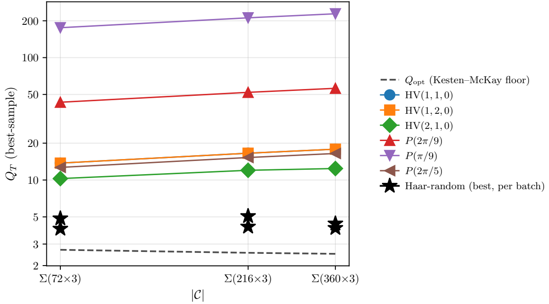
FIG. 2. Q_T across the three \Sigma -series base groups at d = 3 , t = 10 , for every extension in Table III. The dashed line is the Kesten–McKay floor Q_{\text{opt}} . Structured extensions (rational-angle P(\theta) and Howard–Vala) run nearly parallel to it at a factor \sim 3 –70 offset; best-random extensions (stars) approach Q_{\text{opt}} as |\mathcal{C}| grows.
