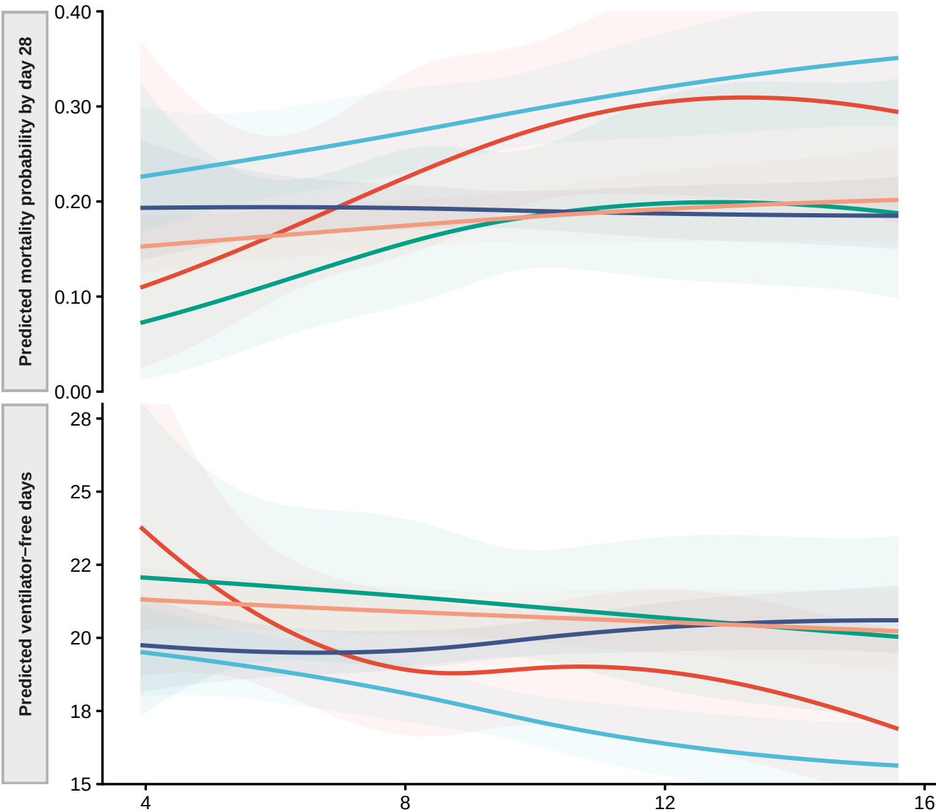
Nitrogen dioxide (NO 2 )
