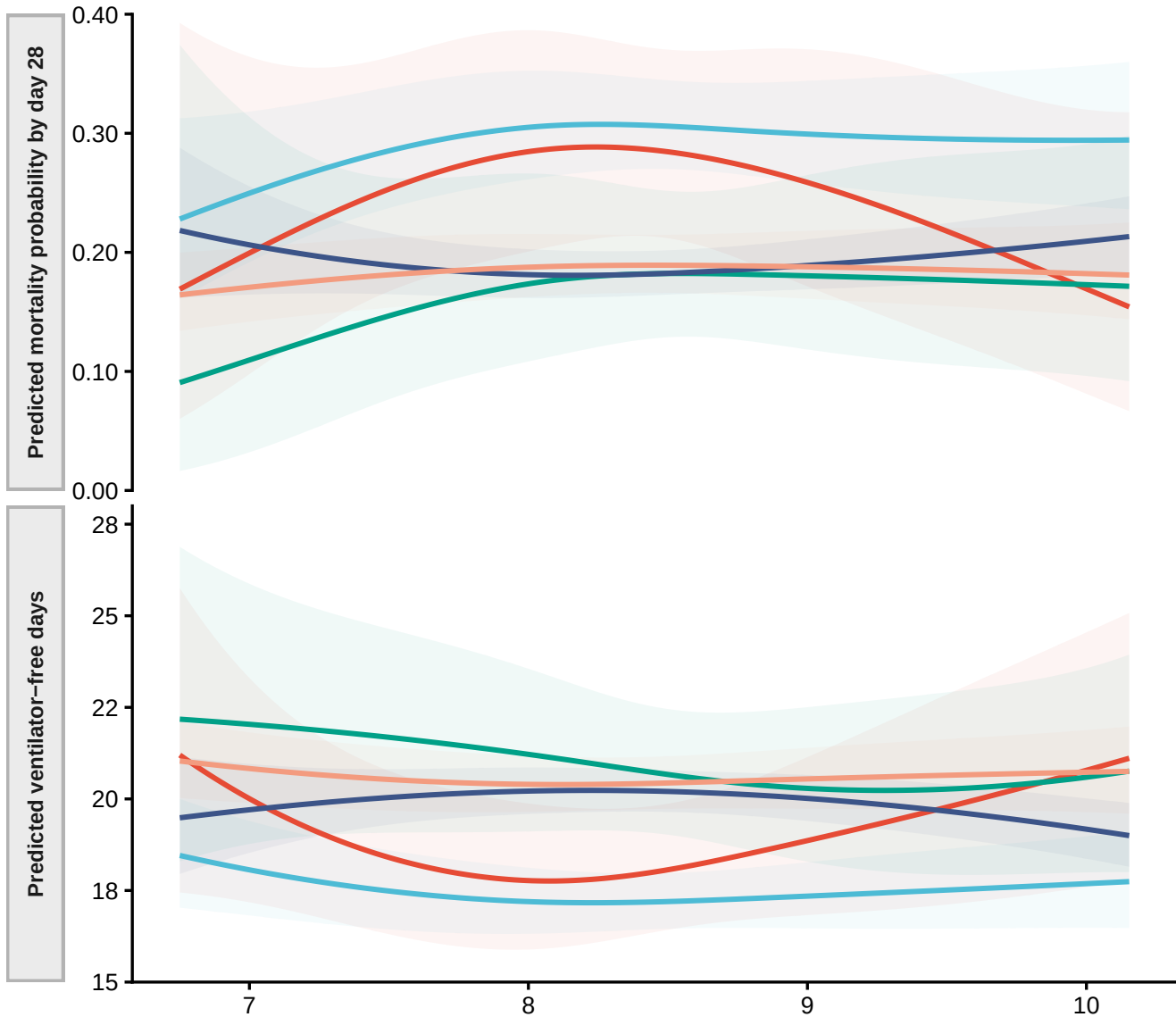
Fine particulate matter (PM 2.5 )
