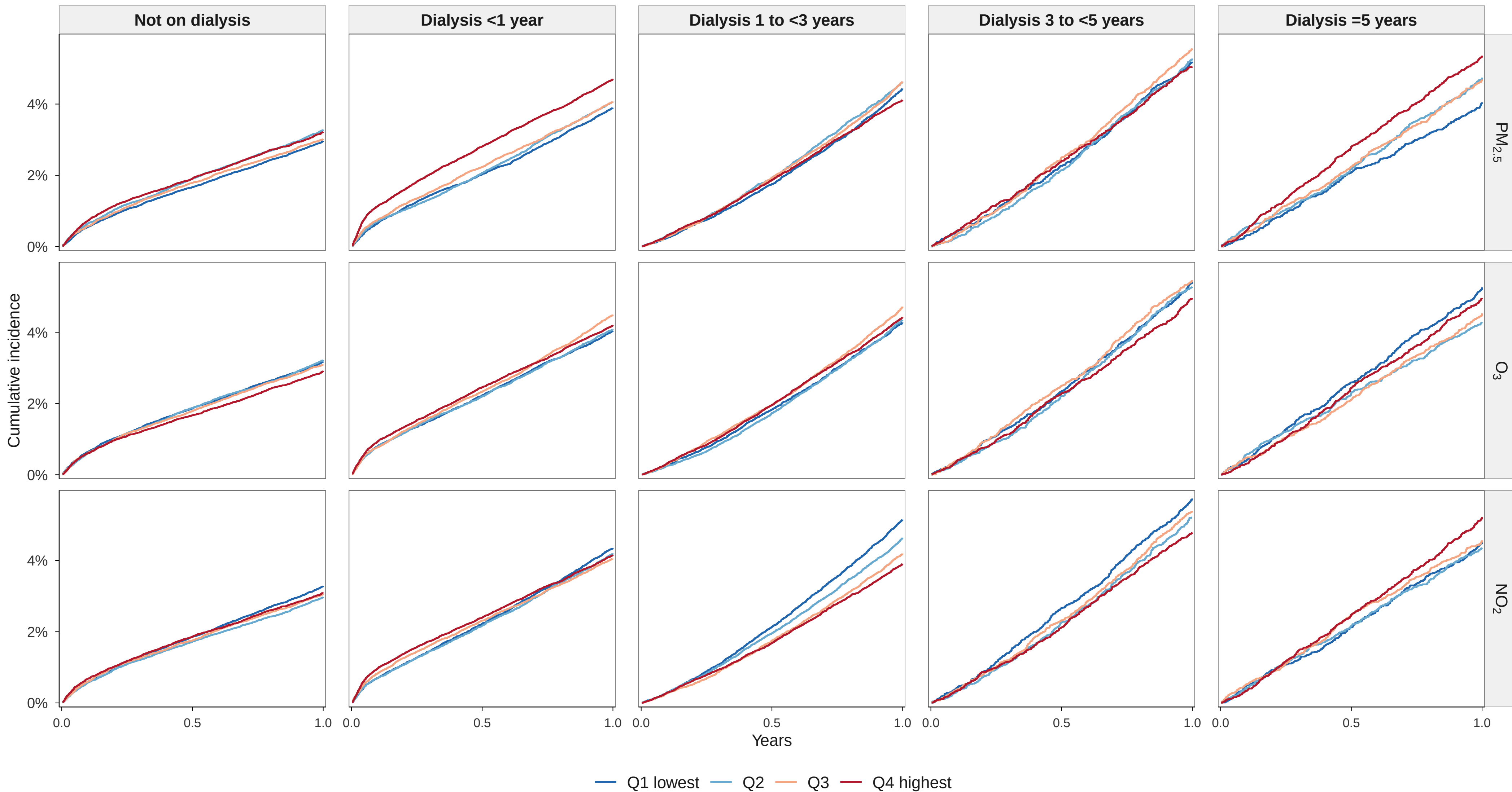
1-Year Cumulative Incidence by Pollution Quartile: Kidney Candidates by Dialysis Vintage at Listing
