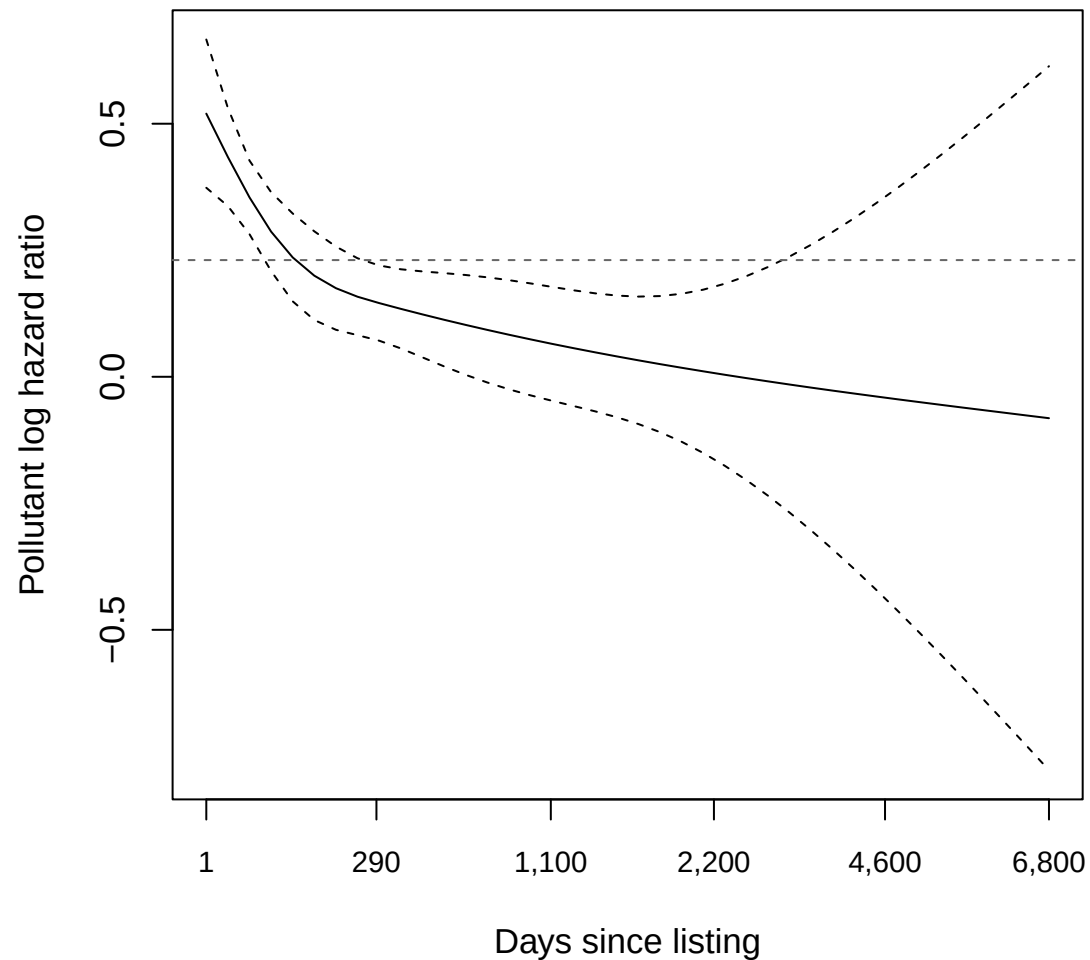
Smoothed coefficient and 95% bands
