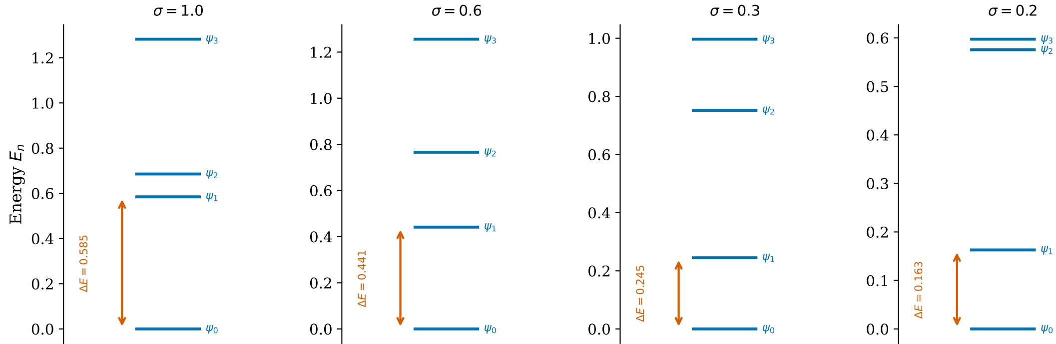
Score Hamiltonian eigenspectrum across diffusion time ( E_0 shifted to 0)
