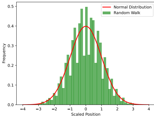
Figure: Central Limit Theorem for One-dimensional Random Walks.
