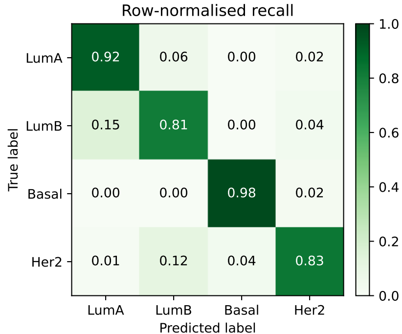
Selective ensemble 10-fold held-out test confusion matrix (986 slides)
