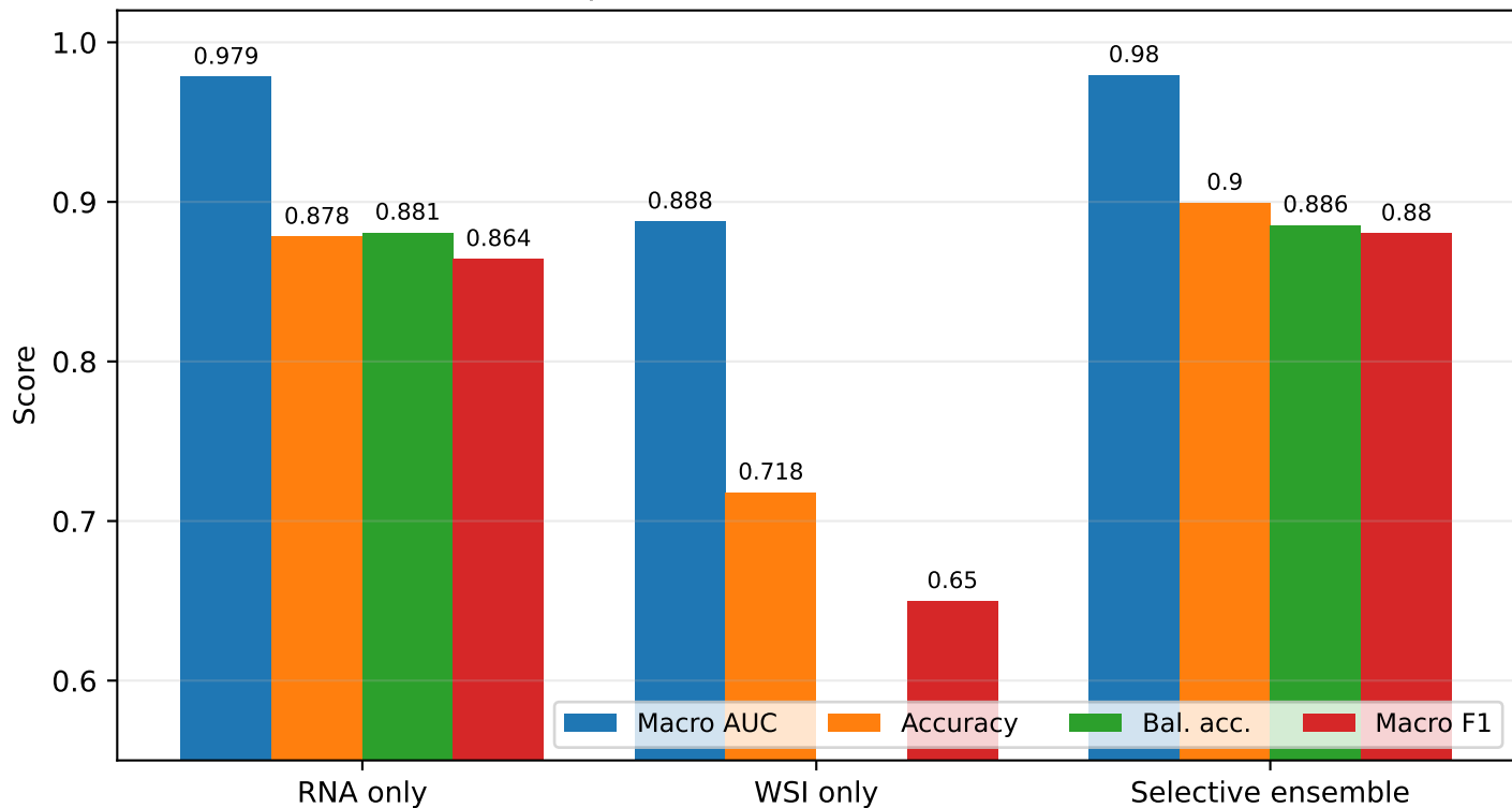
TCGA-BRCA PAM50 performance on the matched 986-slide cohort
