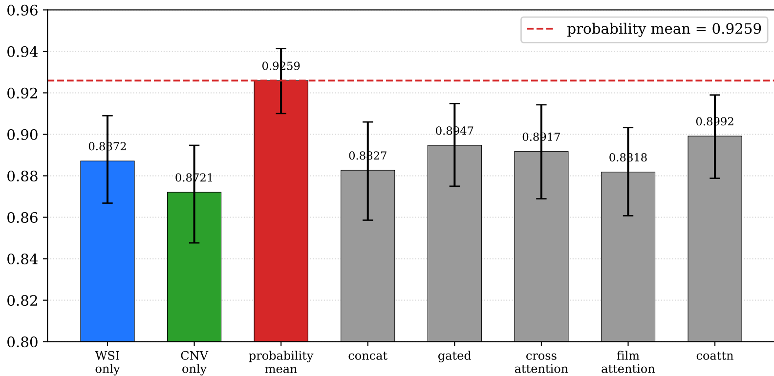
Pooled out-of-fold macro AUROC
