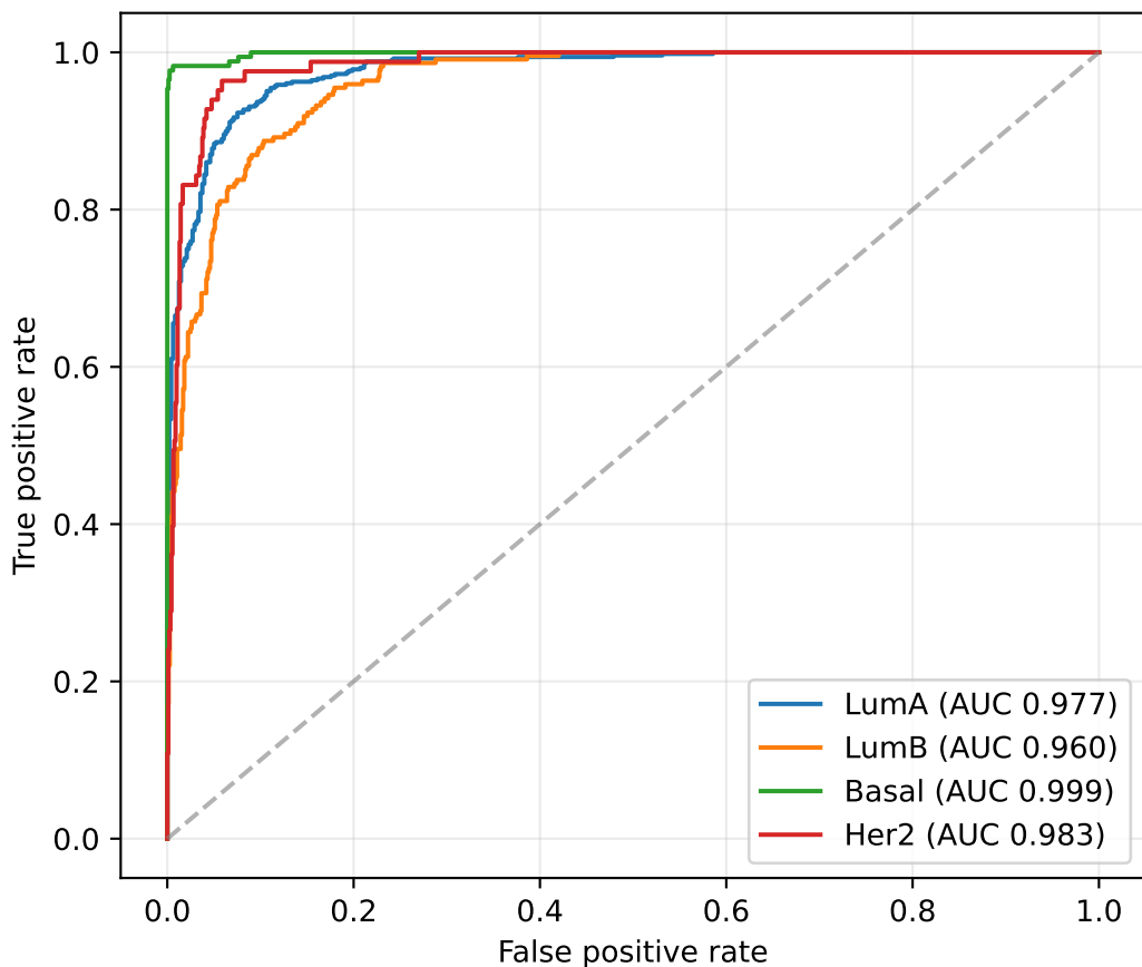
Selective ensemble one-vs-rest ROC curves (986 slides)
