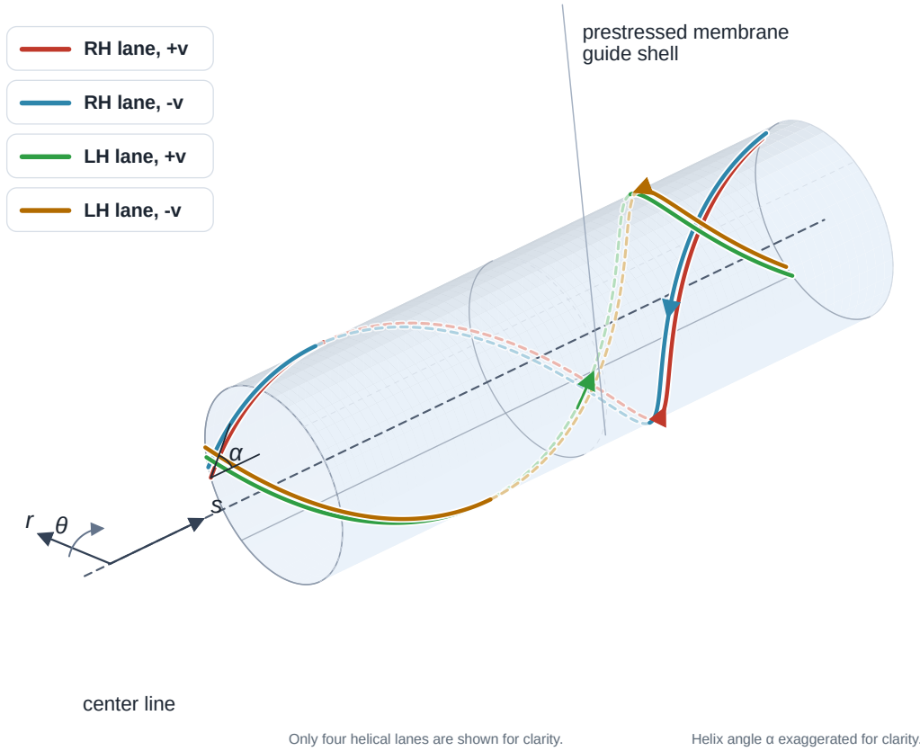
Figure 1b. Local guide-shell segment with representative helical lanes and local coordinates.
