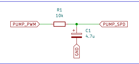
Simulated pump and pump speed sensor
