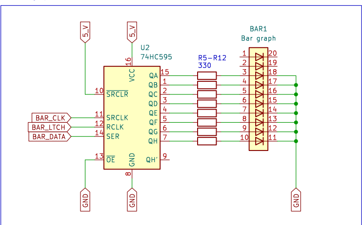
LED bar graph
