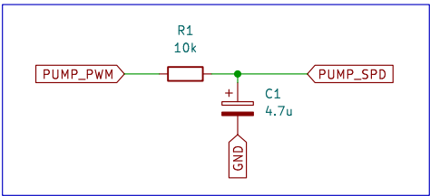
Simulated pump and pump speed sensor
