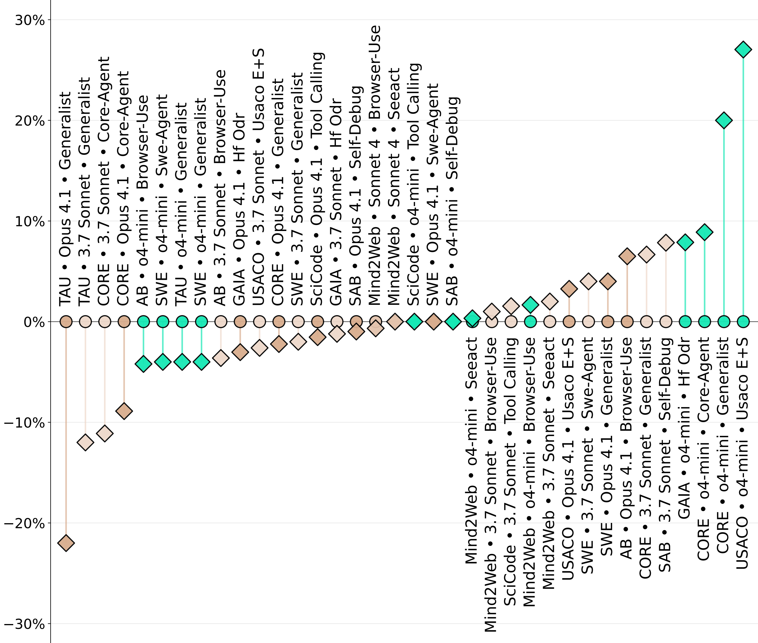
Change in Accuracy From Higher Reasoning Level
