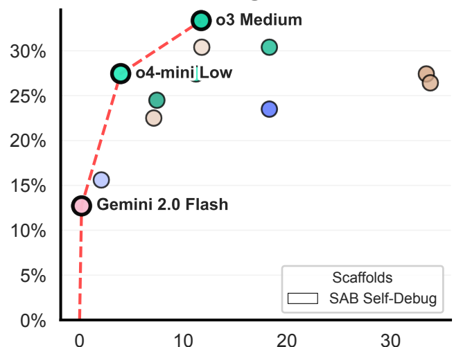
ScienceAgentBench
