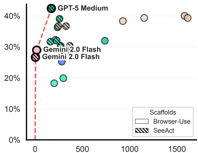
ScienceAgentBench
