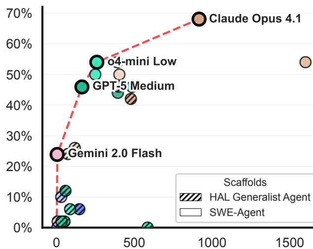
TAU-bench Airline
