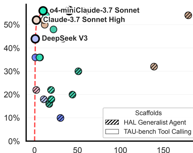
TAU-bench Airline
