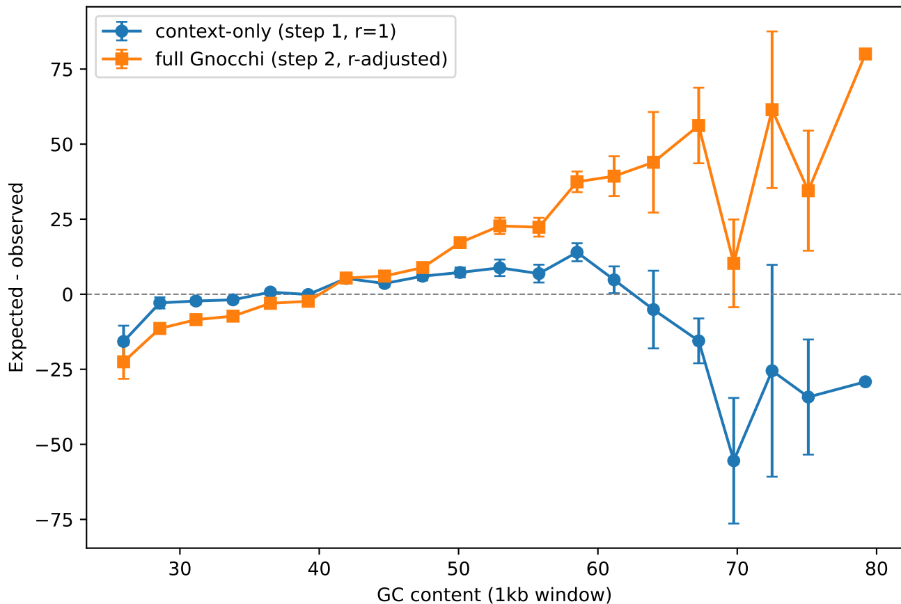
Local mutational bias vs GC content
