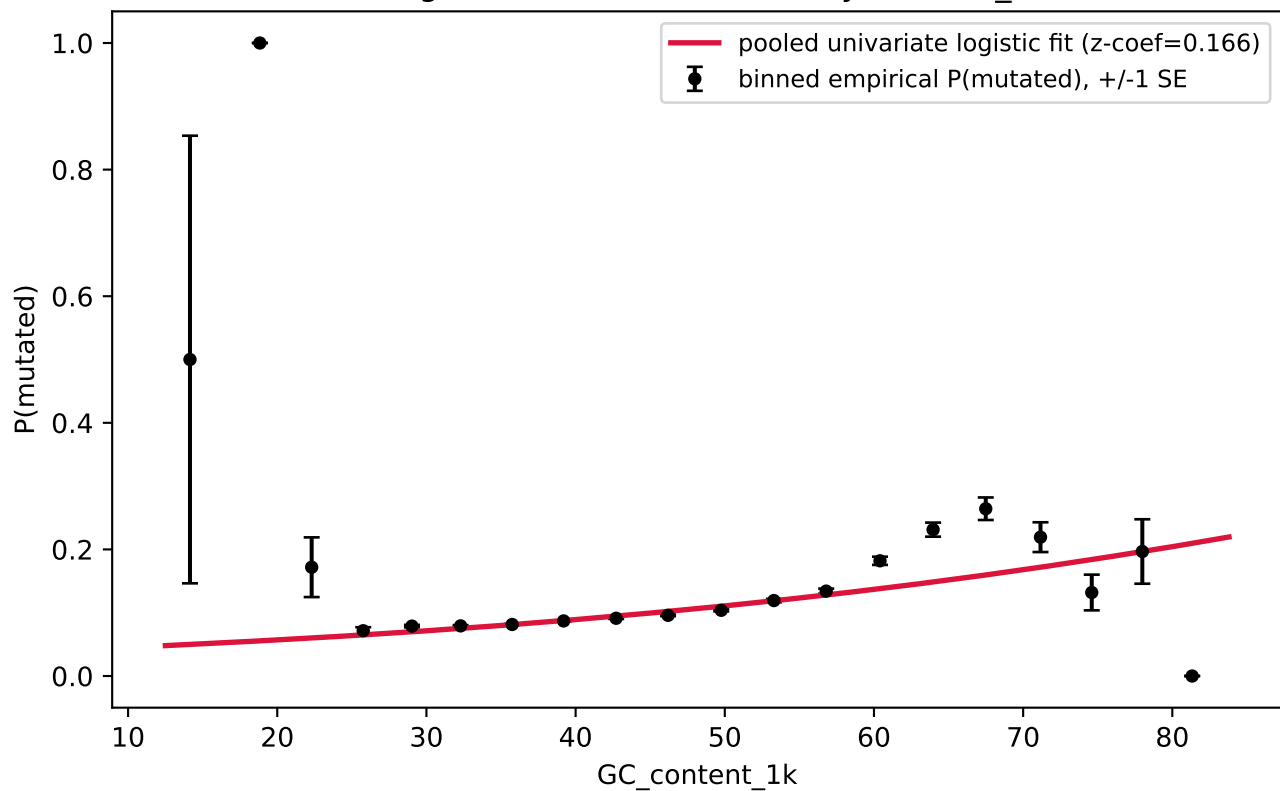
Pooled logistic fit vs GC content only (frac0.1_seed0)
