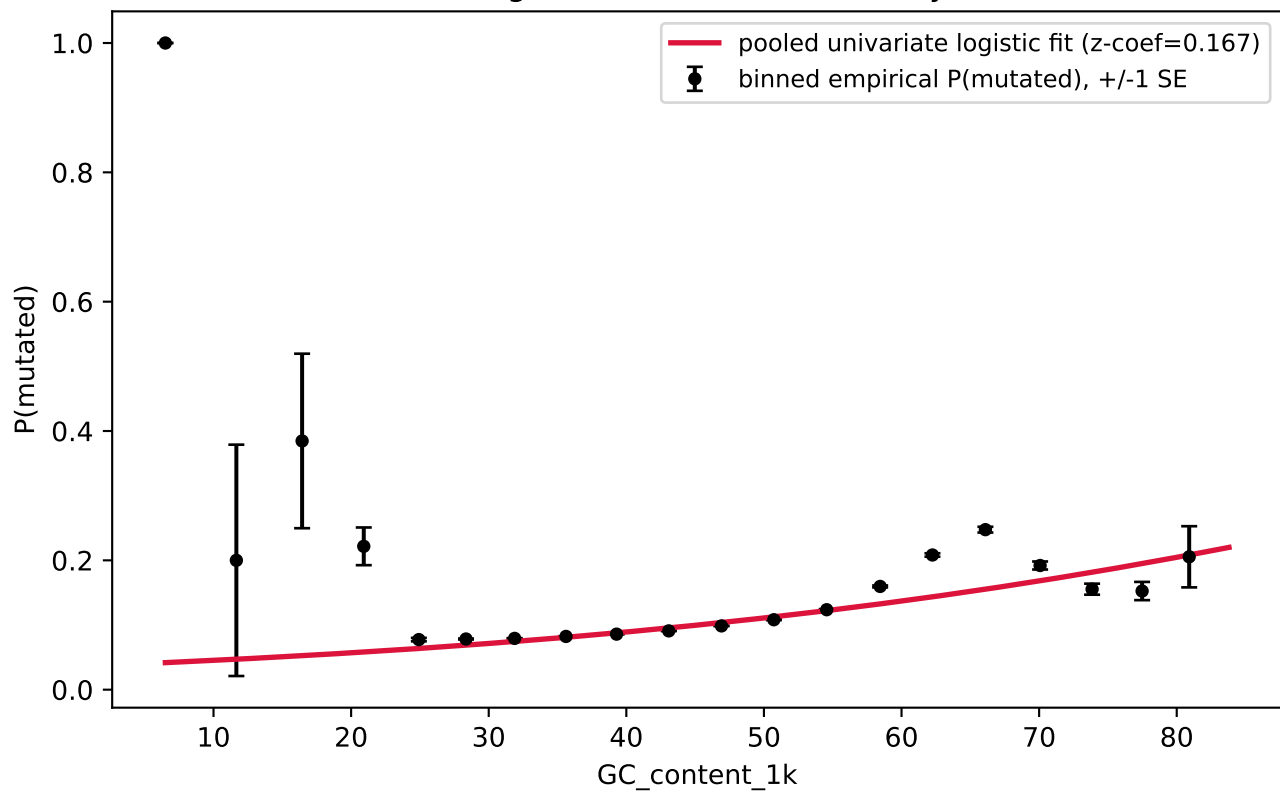
Pooled logistic fit vs GC content only (full)
