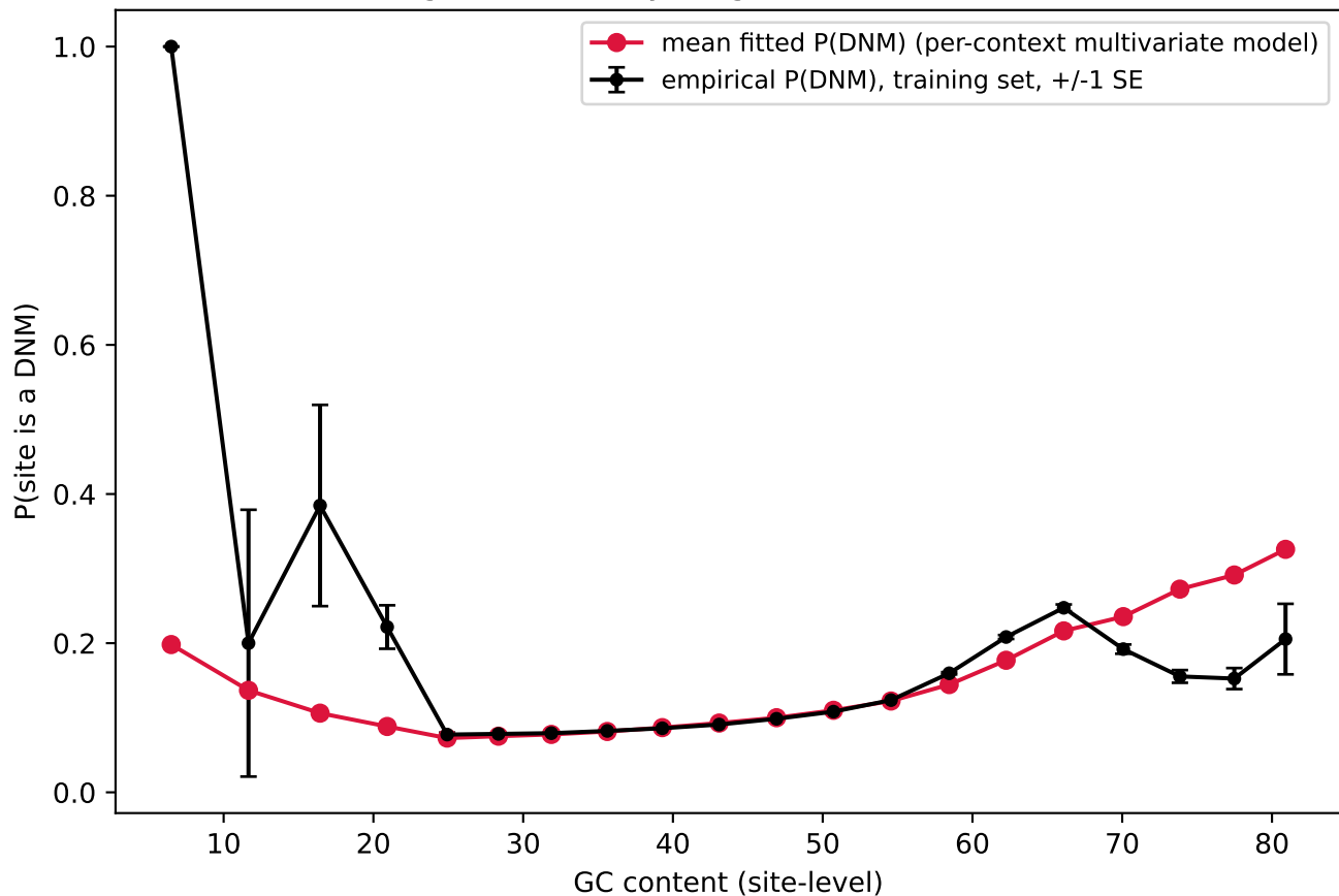
Training-set reliability diagram vs GC content (full)
