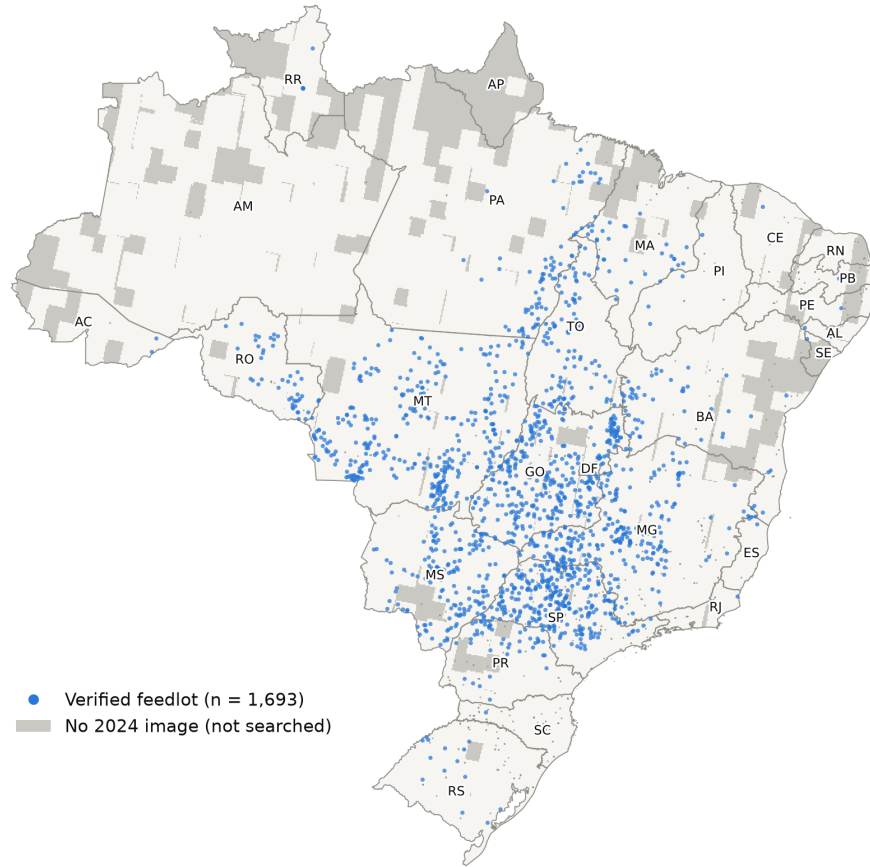
FIGURE A1. Verified feedlots and 2024 image coverage
