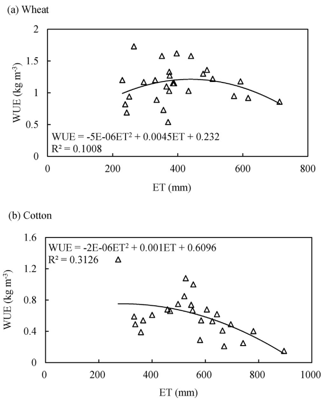
Fig. 4. The WUE-ET relations using the pooled data of (a) wheat and (b) cotton.
