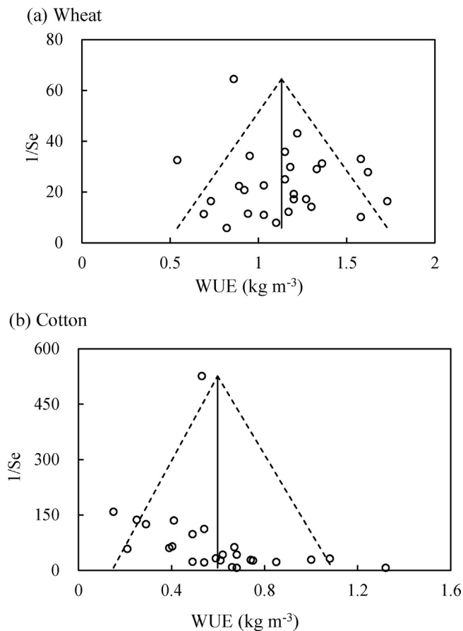
Fig. 5. Funnel plots of WUE using standard errors of (a) wheat and (b) cotton.
