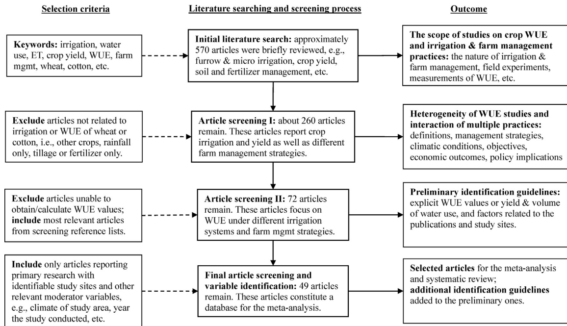
Fig. 1. Literature searching and screening process for selecting sample publications used in the meta-analysis (Adapted from Pagdee et al., 2006).
