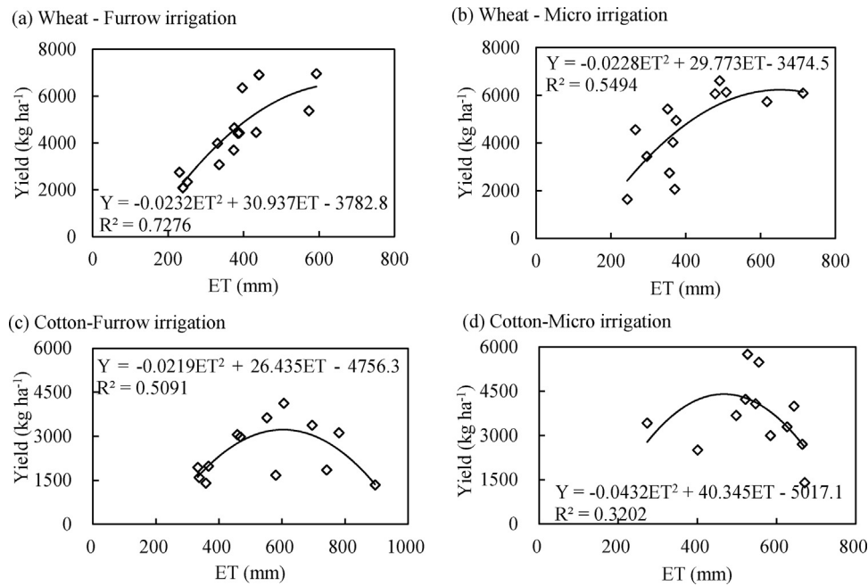
Fig. 2. The yield (Y) and evapotranspiration (ET) relations for wheat and cotton under furrow and micro irrigation systems. For wheat, the grain yield is used to show the yield-ET relation and to calculate WUE, while for cotton, the yield of seed cotton is used.
