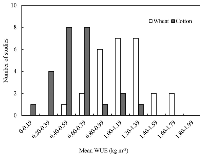
Fig. 3. Histogram of mean WUE of wheat and cotton based on the pooled data of both furrow and micro irrigations.
