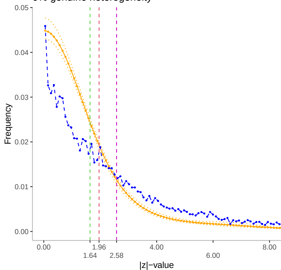
50% genuine heterogeneity
